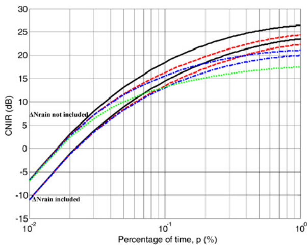
Fig. 10 Tropical location: impact of \Delta N_{\text{rain}} on 19.7 GHz link CNIR for single-polarised system (solid lines) and dual-polarised system: atmospheric depolarisation alone (dotted lines), atmospheric and antennas effect, best-case (dashed-dotted lines), and atmospheric and antennas effect, worst-case (dashed lines) for a 2 m Earth-station antenna at various percentages of time, p
