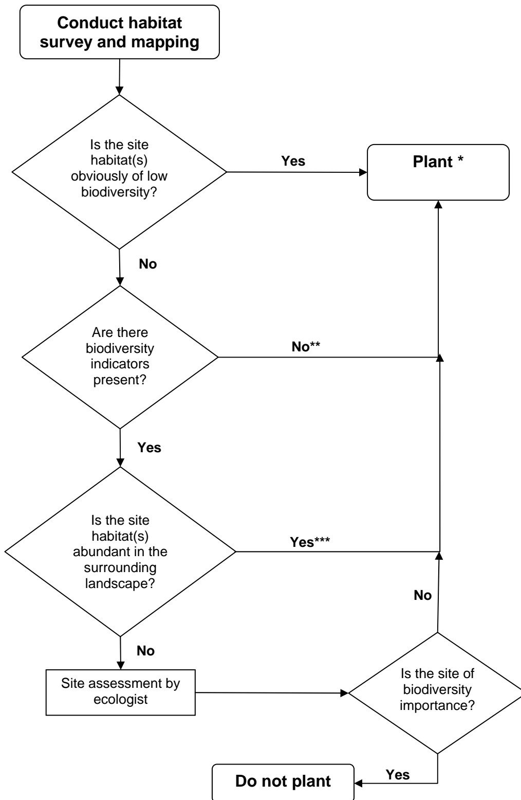
Figure 3. Flow chart outlining the stages in biodiversity assessment prior to afforestation.
