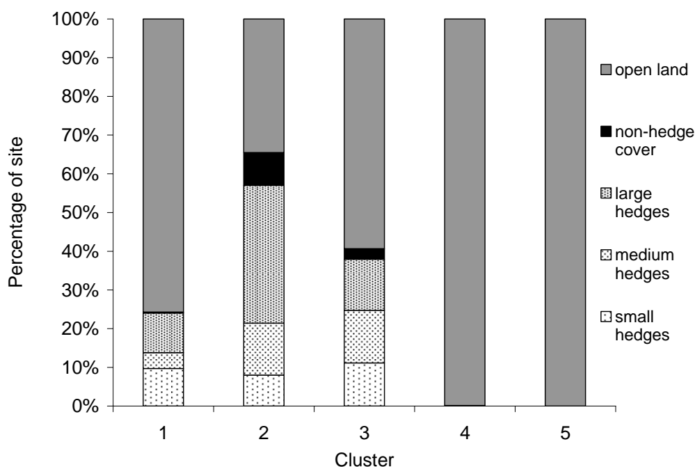
Figure 2. Proportions of cover types in the five bird species clusters. The values for hedge cover shown are the proportions of sites in each cluster within 10m of each of the three hedge categories.
