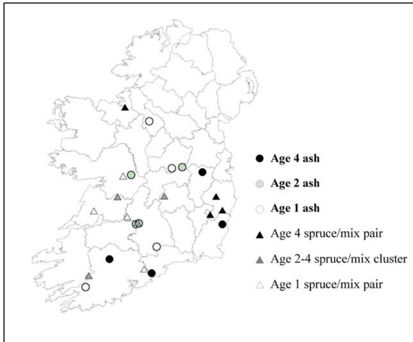
Figure 4. Locations of study sites for Project 3.1.2.
