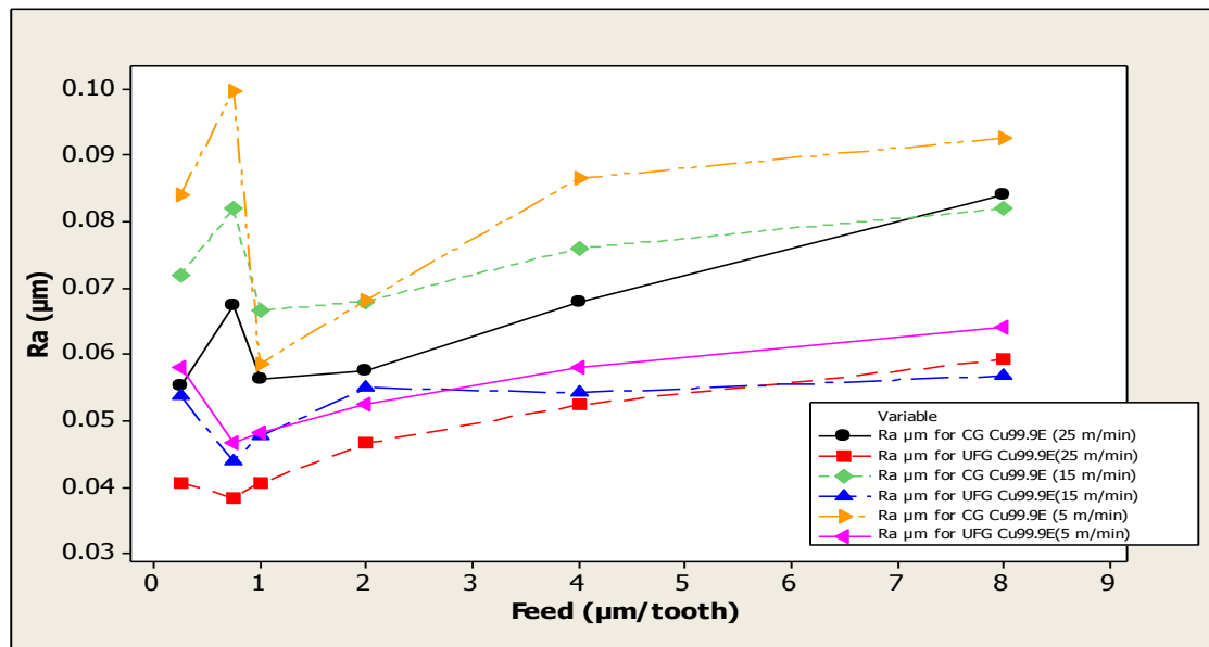
Fig. 8: Roughness achieved under different cutting conditions for CG and UFG Cu99.9E
