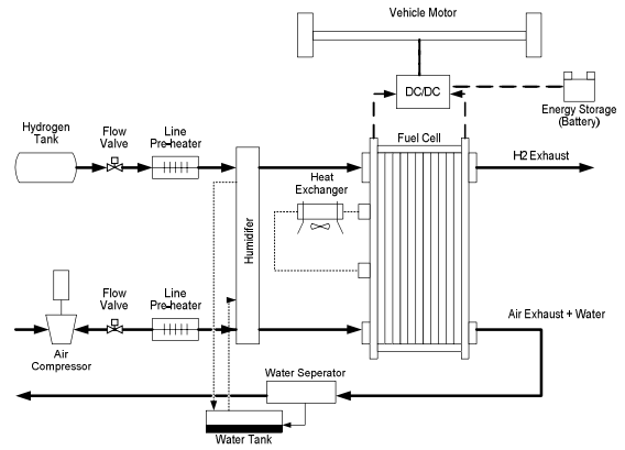
Figure.2 An overall configuration of fuel cell vehicle
