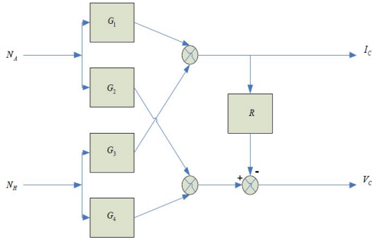
Figure.1. MIMO representation of fuel cell
