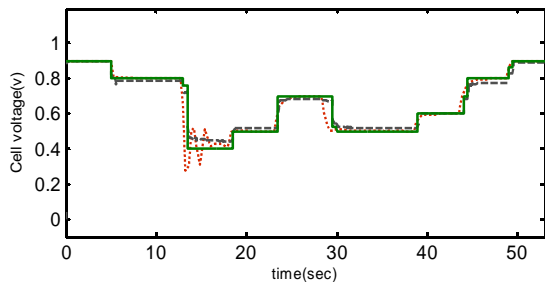
Figure 3. The responses of cell voltage Using a PID controller (Ref — PID — — mfc ····)
