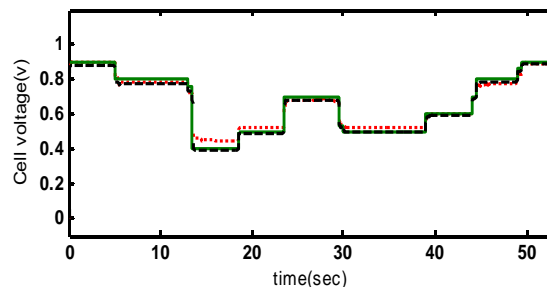
Fig.5. Comparison of simulation responses of cell voltage using a PID and Fuzzy-PID hybrid controllers for set point changes (Ref — Hybrid Control — — PID Control ····)
