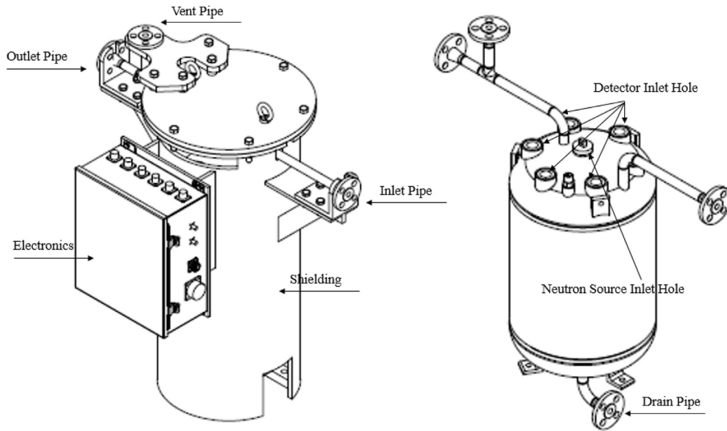
Fig. 1. Schematic of sample assembly (left) and pressure vessel (right).
