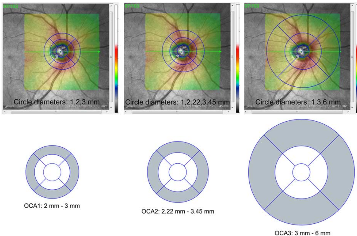
FIGURE 1. Schematic representation and definition of the outer circumpapillary annuli (OCA1, OCA2, OCA3) of circular grids 1, 2, and 3. The upper row shows the infrared reflectance images of the optic nerve and peripapillary region. In the infrared reflectance images, the transparent colored areas which are centered over the optic nerve represent the 20 × 20 degree region scanned in the 3-dimensional volume scan. The blue circular grids are manually centered over the optic nerve from which the machine’s internal software generates the retinal volume values. Images in the lower row shows the diameters of OCA1, OCA2, OCA3 used in this study.
