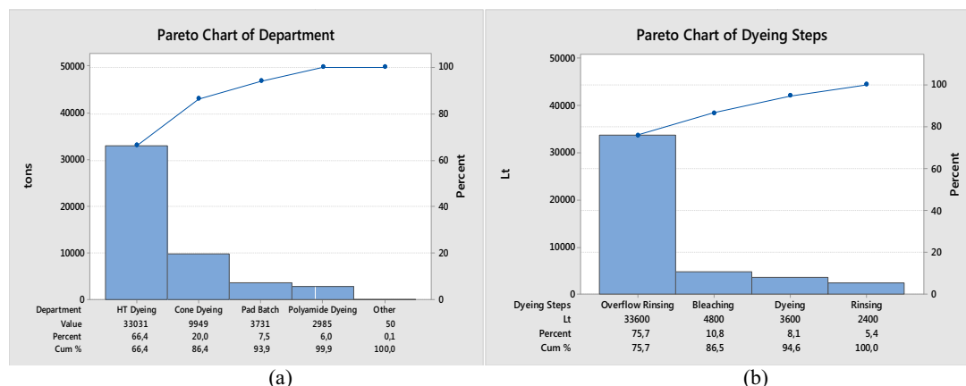
Fig 1. Minitab Pareto analysis results (a) for water consumption ratios of dye house departments,(b) for water consumption ratios of reactive dyeing process
