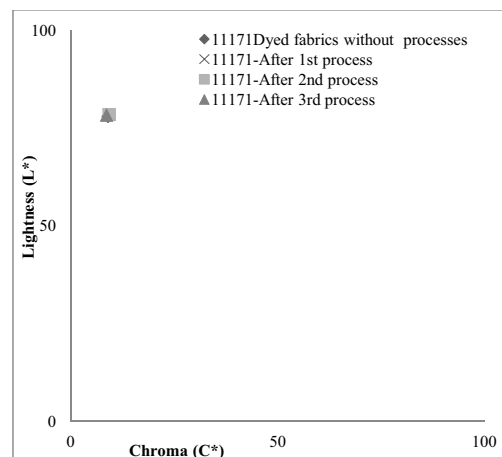
Fig 5. L^* (Lightness)- C^* (Chroma) values of samples
