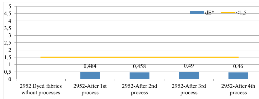
Fig 6. Color differences ( \Delta E ) values of samples
