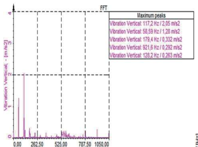
Fig. 5. Spectrum in vibration FFT data of radial direction
