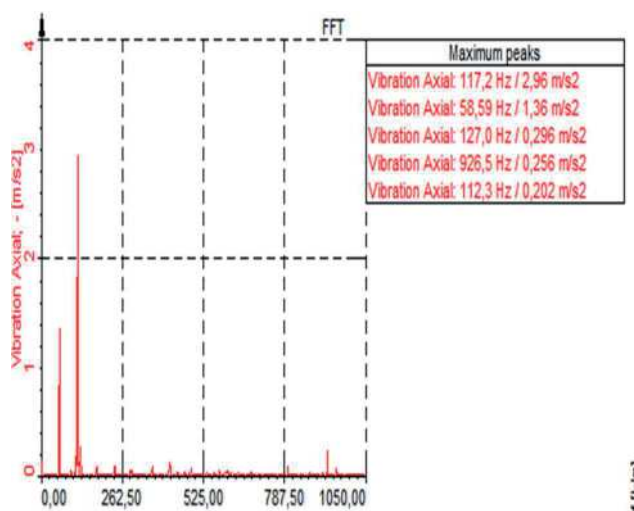
Figure 6. Spectrum in vibration data of axial direction
