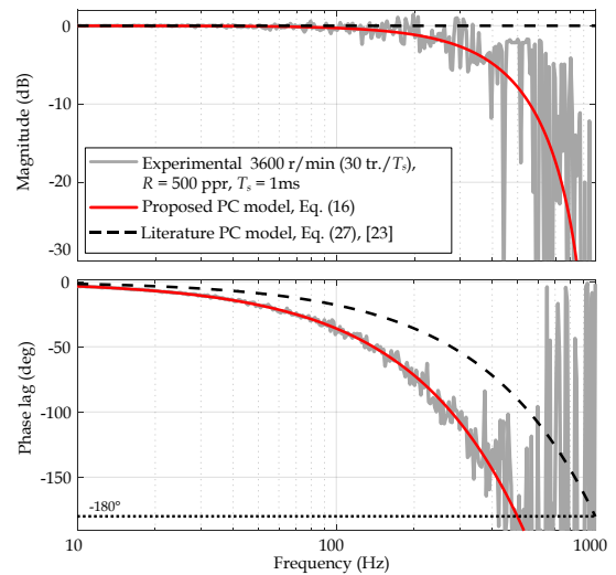
Fig. 8 Experimental validation and comparison of the PC models.
