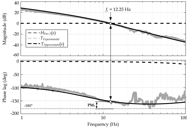
Fig. 13 Experimental frequency response of the loop gain of the dc motor system at 500 r/min (0.42 tr./ T_s )
