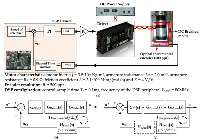
Fig. 12 (a) Diagram of the dc motor system, (b) block diagram of the system and (c) compensated block diagram.
