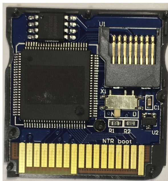
Fig. 2. Inside the R4i.
