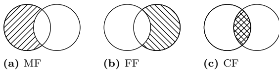
Fig. 10. Friends adversarial models (hashed area) for user i : (a) My other friends model (MF); (b) My friend's other friends model (FF); (c) Our friends in common model (CF). The social circle of user i (resp. j ) is represented by the left (resp. right) circle. The intersection represents the common friends of i and j .
