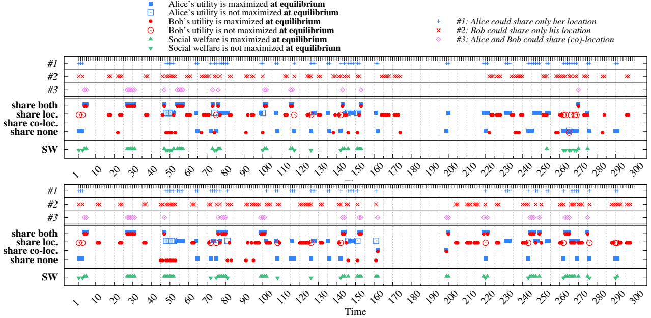
Fig. 5. Possible strategies and equilibria decisions (CF adversarial model) when Alice and Bob use two random traces from the Geolife dataset, for f_{sv} = 0.57 , f_{lc} = 0.56 , f_{pb} = 0.60 . We illustrate the game outcome between Alice and Bob in two cases: 7% (top) and 10% (bottom) co-locations, respectively – the trace used by Alice is exactly the same in both cases. The x axis shows the entire time window of interest. In the top section, on the y axis, the possible strategies at each time instant of the game are illustrated: Alice can only share location (blue ‘plus’), Bob can only share location (red ‘cross’), Alice and Bob can both share location and co-location (violet ‘rhombus’); For time instants where the game cannot be played (missing location data) there is no symbol. The middle and bottom sections of the y axis illustrate the equilibria decisions : For every time instant, Alice’s decision is represented by a blue rectangle and Bob’s decision by a red circle; A player’s corresponding shape is full if its utility at equilibrium is maximized, and empty otherwise. Additionally, each time instant at which both Alice and Bob can play is marked by an upward-pointing green triangle, if the equilibrium decisions maximize social welfare or by a downward-pointing green rectangle if they do not.
