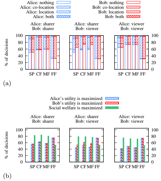
Fig. 8. Equilibria decisions (a) and their properties (b), when Alice and Bob have different preference profiles, corresponding to real survey data: 150 sharers ' profiles ( f_{sv} > 0.5 ) and 58 viewers ' profiles ( f_{sv} < 0.5 ). We present three scenarios: both Alice and Bob are sharers (left plots), Alice is a sharer and Bob is a viewer (middle plots) and both are viewers (right plots). Note that, due to the symmetry of the trajectories in the meeting scenario, the case where Alice is a viewer and Bob is a sharer is symmetric to the case where Alice is a sharer and Bob is a viewer . Different adversarial models (SP, CF, MF, FF) are illustrated on the x axis. In each of the top three plots, for each adversarial model, two bars (blue on the left for Alice and red on the right for Bob) indicate—on the y axis—the proportion of times (aggregated over time instants and the number of preference profile pairs considered in that scenario) a player made one of the four possible decisions: share nothing (empty pattern), share only location (hash right pattern), share only co-location (hash left pattern) or share both (hash right-left pattern). Each of the three bottom plots show, on the y axis, for each adversarial model, the proportion of times social welfare and individual utilities are maximized.
