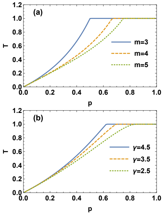
FIG. 2: The percolation probability T is plotted versus p for deterministic hyperbolic manifolds with m = 3, 4, 5 (panel a) and random hyperbolic manifolds with scale-free distribution q_m = Cm^{-\gamma} with m \geq 3 and \gamma = 4.5, 3.5, 2.5 .
