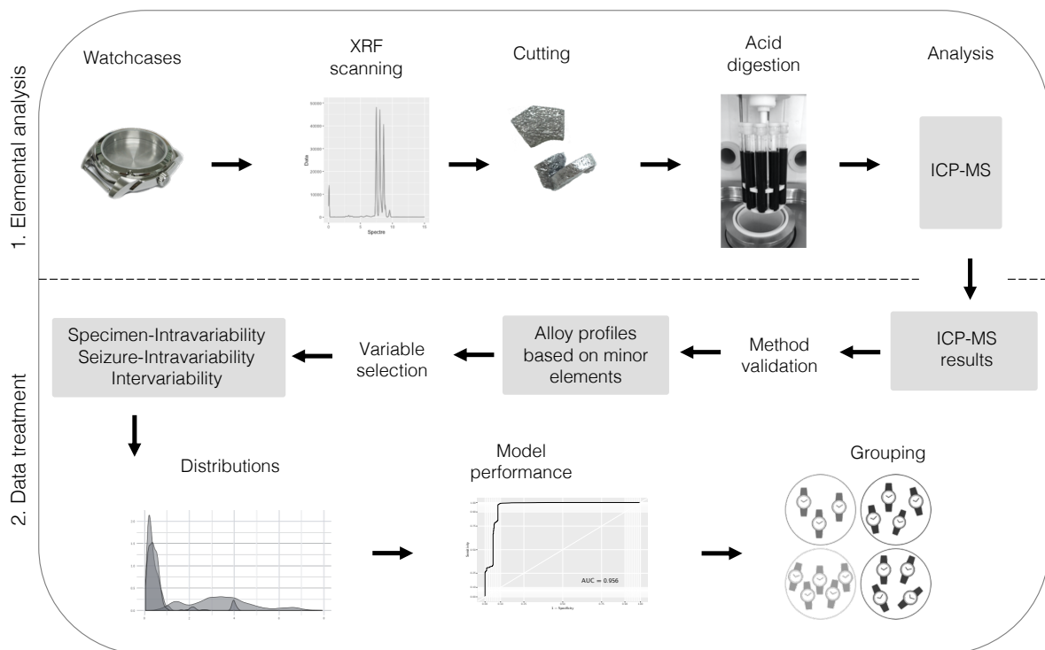
Figure 3: Elemental analysis process and data treatment for the chemical profiling
