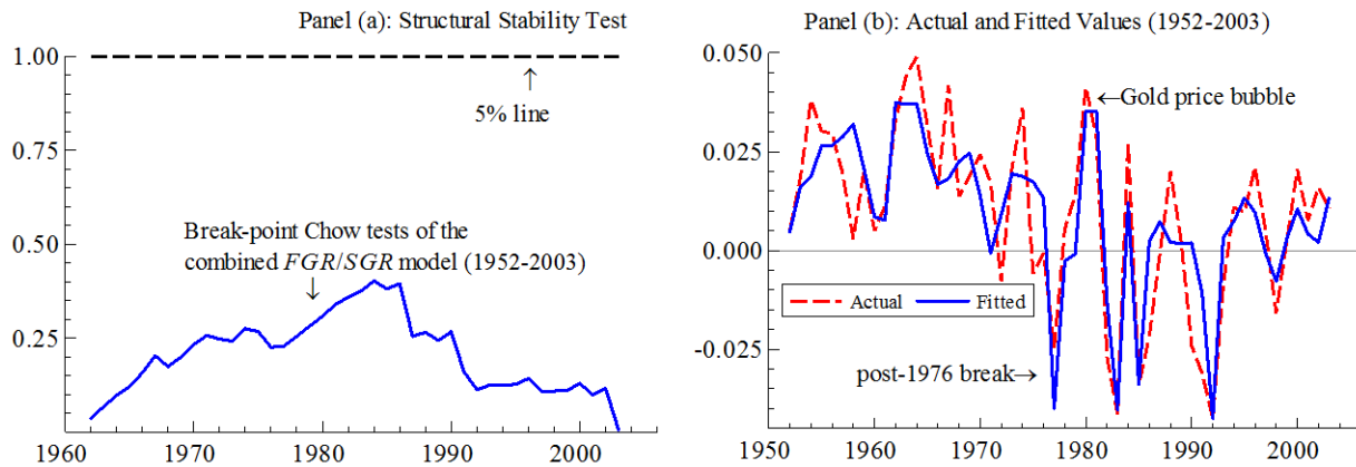
Figure 5: Structural Stability Test and Fitted Values
