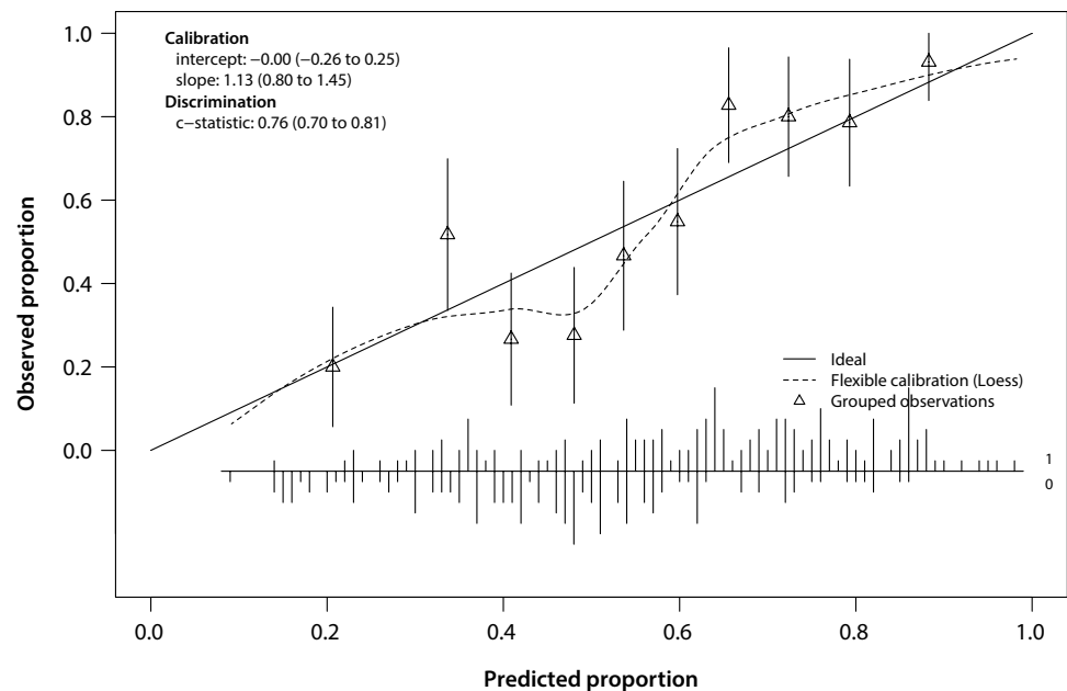
Fig. 1 Calibration plot of the prediction model for beneficial fKSS outcomes fitted to the individual data of 295 patients. The triangles represent the observed percentages versus the predicted probabilities of responding. The vertical lines represent the 95% CI of the observed probabilities. The broom plot at the bottom shows the distribution of predicted probabilities separately for patients with and without a beneficial functional outcome
