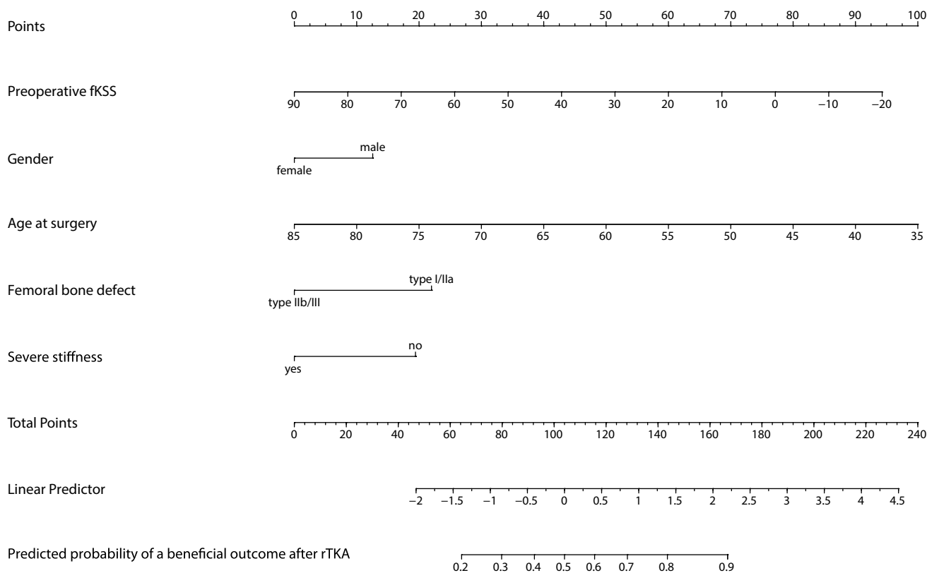
Fig. 2 Nomogram for prediction of a beneficial functional outcome 5 years after rTKA in a given patient. To obtain the predicted probability of a beneficial outcome, (1) Locate the patient's values for "Preoperative fKSS", "Gender", "Age at surgery", "Femoral bone defect", and "Severe stiffness" on the corresponding axes, (2) Draw a vertical line from the located value on each axis to the "Points"-axis to determine how many points are attributed for each predictor, (3) Sum the points for all variables, (4) Locate the sum on the "Total Points"-axis, and (5) Draw a vertical line towards the "Predicted probability of a beneficial outcome after rTKA"-axis to determine the probability of a beneficial functional outcome 5 years after rTKA. To illustrate the use of the nomogram, the outcome for a 65-year-old female patient with a preoperative fKSS of 50 who has a type IIb AORI femur bone defect, and severe stiffness as main reason for revision is predicted.
