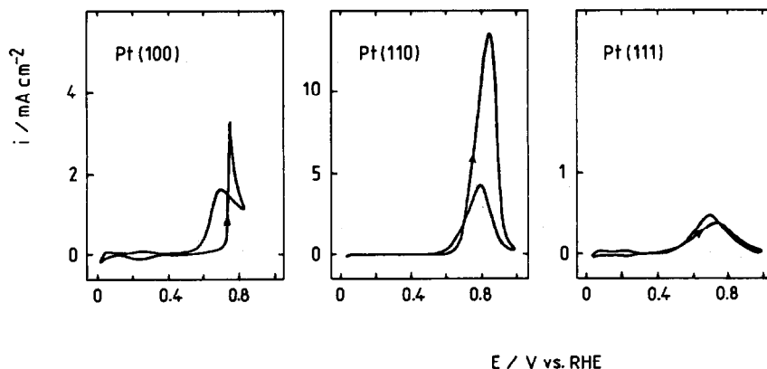
Fig. 9. Voltammograms of Pt(100), Pt(110) and Pt(111) single crystal electrodes in 0.5\text{ M HClO}_4 + 0.1\text{ M CH}_3\text{OH} solutions at 25^\circ\text{C} and \nu = 50\text{ mV s}^{-1} ; only the first sweep is represented.
