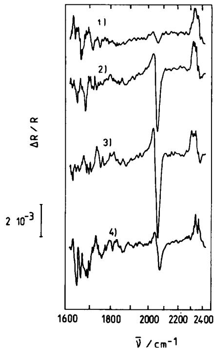
Fig. 12. EMIRS spectra of the adsorbed species resulting from the chemisorption of 1 M \text{CH}_3\text{OH} in 0.5 M \text{HClO}_4 at a rough Pt electrode. f = 13.5 Hz; 10 averaged scans. \Delta E = 400 mV; potential pulse centre (V vs rhe ): (1) = 0.2; (2) = 0.3; (3) = 0.4; (4) = 0.5.
