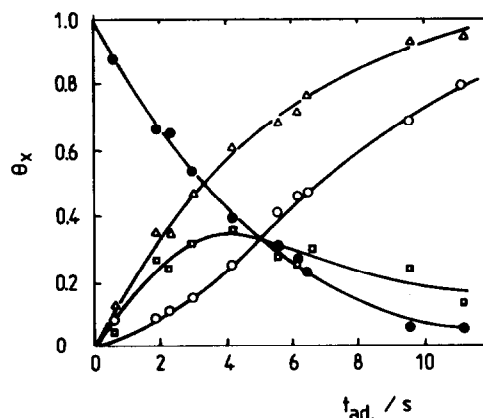
Fig. 2. Adsorption of CO on a pc. Pt electrode immersed in a 1 M HClO 4 solution saturated with gaseous CO. The degree of surface coverage, \Theta , by the two adsorbed species, CO L and CO B , is given as a function of t_{ad} . E_{ad} = 0.59 \text{ V/rhe} , 25^\circ\text{C} : ( \bullet ) \Theta_H ; ( \square ) \Theta_{CO}^B ; ( \circ ) \Theta_{CO}^L ; ( \triangle ) \Theta_{CO}^T = \Theta_{CO}^B + \Theta_{CO}^L .
