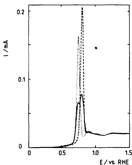
Fig. 4. Voltammograms of adsorbed CO electrooxidation on polycrystalline(—), type I (· · ·) and type II (---) platinum electrodes. Adsorption potential E_{\text{ad}} = 0.25 \text{ V/rhe} ; adsorption time t_{\text{ad}} = 1 \text{ min} , sweep rate, v = 0.1 \text{ V s}^{-1} ; 0.05 M \text{HClO}_4 ; 25°C. For the preparation of type I and type II electrodes[18].
