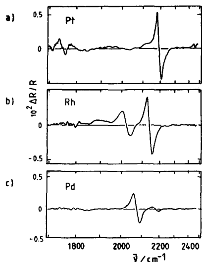
Fig. 5. EMIRS spectra of CO species adsorbed on noble metal electrodes immersed in a 0.5 M \text{HClO}_4 solution saturated with gaseous CO. \Delta E = 400 mV, \bar{E} = 0.2 V vs r.h.e., f = 13.5 Hz: (a) Pt; (b) Rh; (c) Pd.
