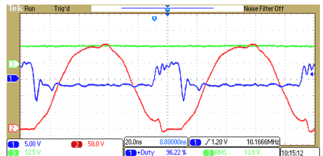
Fig. 22. Experimental waveforms for V_{in}=254 V, Phase-shift \Phi_{p-s}=35 ns ( 126^\circ ), D_{pri}=18\% . CH1: Gate-to-source signal of S_2 [5 V/div]; CH2: Drain-to-source waveform of S_2 [50 V/div]; CH3: Output voltage across 40 Ω load [12.5 V/div].
