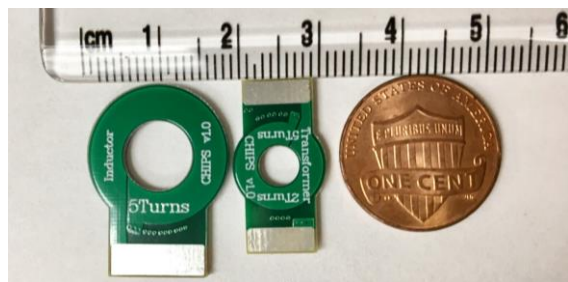
Fig. 10. A photo of inductor and transformer PCB winding prototypes.
