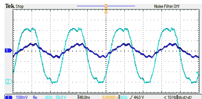
Fig. 21. Experimental waveforms for V_{in}=254 V, Phase-shift \Phi_{p-s}=25 ns ( 90^\circ ), D_{pri}=18\% . CH1: Resonant tank current [2 A/div] (dark blue); CH2: Resonant tank voltage [50 V/div] (light blue).
