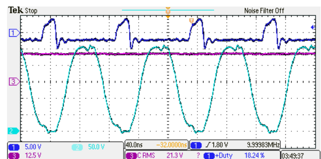
Fig. 20. Experimental waveforms for V_{in}=254 V, Phase-shift \Phi_{p-s}=25 ns ( 90^\circ ), D_{pri}=18\% . CH1: Gate-to-source signal of S_2 [5 V/div]; CH2: Drain-to-source waveform of S_2 [50 V/div]; CH3: Output voltage across 40 Ω load [12.5 V/div].
