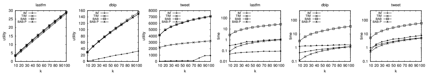
Fig. 4: Varying number k of promoters.
