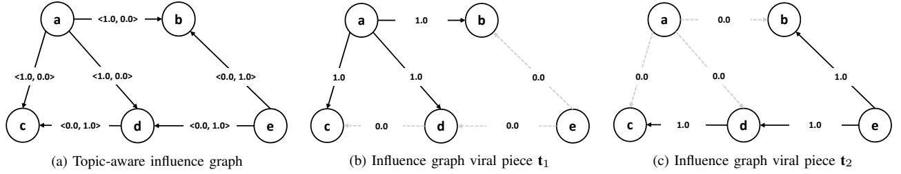
Fig. 1: A running example for \mathcal{OIIPA} . In (a), each edge in contains a topic-aware influence probability vector. In (b), we show the influence graph for \mathbf{t}_1 which has a topic distribution of (1, 0) . In (c), we show the influence graph for \mathbf{t}_2 which has a topic distribution of (0, 1) .
