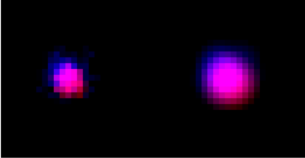
Figure 7. Two-color images illustrating the offset between the hard (1.5–7.3 keV, blue) and soft (0.45–1.1 keV, red) central PSFs for the combined 2010 observations. Left : unsmoothed, 1 pixel = 0.125". – Right : smoothed using Gaussian of width = 3 pixels, 1 pixel = 0.125".
