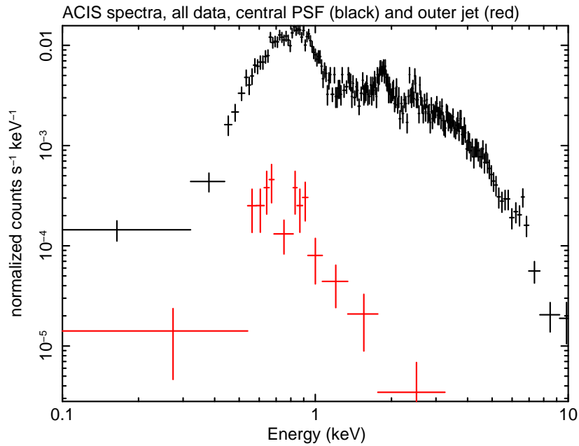
Figure 6. Spectrum of central Chandra PSF (black) and the outer, resolved jet (red). All available Chandra data were combined. Note similarity between jet spectrum and the soft peak of the central-PSF spectrum.
