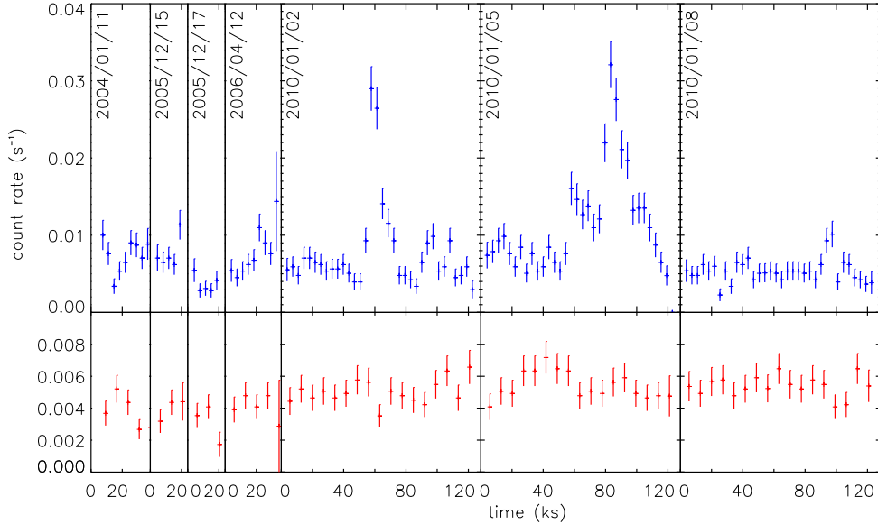
Figure 4. Hard (1.5–7.3 keV, upper panel) and soft (0.5–1.0 keV, lower panel) light curves extracted from the central PSF of all Chandra DG Tau observations; the individual observations are separated by vertical lines, and observing dates are given in the upper panels. Note the absence of correlated behavior in the two light curves and the nearly constant flux level in the soft emission except for a gradual increase in luminosity over 6 years, from 1.1 \times 10^{29} erg s ^{-1} to 1.8 \times 10^{29} erg s ^{-1} .
