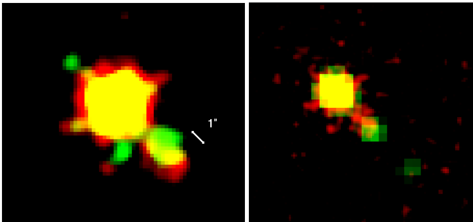
Figure 2. Left (a): Two-color image, showing superposition of smoothed X-ray images for Winter 2005/06 (green) and for January 2010 (red), indicating jet longitudinal motion. – Right (b): Calar Alto Potsdam Multi Aperture Spectrophotometer (PMAS) [S II] image (green) superimposed on a smoothed X-ray image (red).
