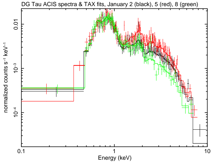
Figure 5. Chandra ACIS-S spectra of the DG Tau X-ray source in the central PSF. The spectra refer to observations taken on January 2 (black), January 5 (red), and January 8 (green), 2010. Note variability above 1.5 keV due to flares (see Fig. 4), but identical spectra below \approx 1.2 keV.
