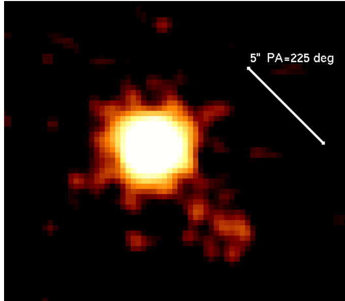
Figure 1. X-ray jet of DG Tau observed in January 2010, in the energy range 0.4–1.5 keV; the original data have been smoothed using a Gaussian kernel of width 1.2 pixels, where 1 pixel = 0.25".
