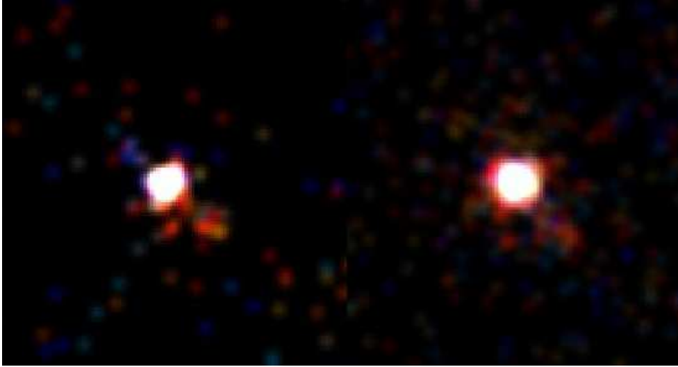
Figure 3. Smoothed hardness images of the DG Tau jet in 2004-2006 (left) and 2010 (right). Red is softest, blue hardest (for photons ranging from 0.5-1.5 keV). Note the absence of a significant counter-jet in 2010.
