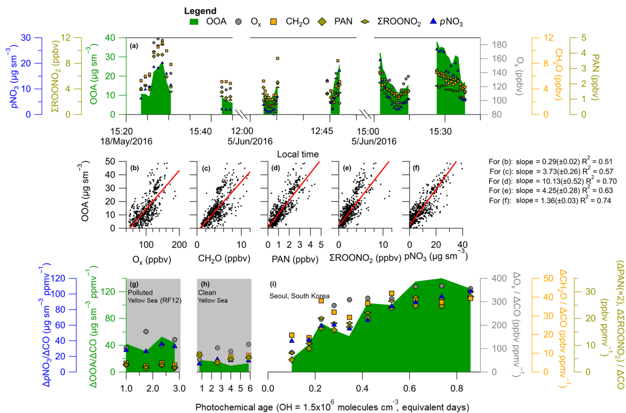
Figure 7. (a) Time series of OOA (OOA = LO-OOA + MO-OOA), O x , CH 2 O, PAN, ΣROONO 2 , and pNO 3 during RF09 (18 May 2016), and RF18 (5 June 2016) noon and afternoon overpasses. Gaps in time series correspond to climbing out of the boundary layer. OOA versus (b) O x (O x = O 3 + NO 2 ), (c) CH 2 O, (d) PAN, (e) ΣROONO 2 , and (f) pNO 3 over Seoul, South Korea, during KORUS-AQ. For (b)–(f), the observations are after 12:00 LT (03:00 UTC), the black dots are all data, and the slopes (red line) are an ODR fit to the data. (g–i) Same as Fig. 6 for ΔOOA/ΔCO versus photochemical age, and including the dilution-corrected production of O x , CH 2 O, PAN, ΣROONO 2 , and pNO 3 . Panel (g) shows observations over the Yellow Sea (RF12), (h) over the Yellow Sea (normal conditions), and (i) over Seoul. Similar to Fig. 4, the Δ corresponds to subtracting the background values for the respective species.
