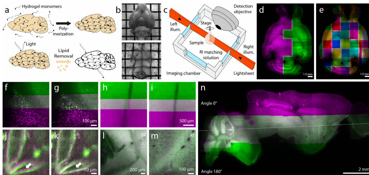
Figure 1 | BigStitcher Principles. (a) schematic of the CLARITY sample clearing process. (b) adult mouse brain before (up) and after (down) clearing. (c) the layout of the type of lightsheet microscope used for acquisition [beads] (d) single slice through an entire adult mouse brain acquired with dual-sided illumination. Pink (left illum.) and green (right illum.) image tiles highlight the illumination direction that was automatically selected for each tile. (e) overview of an entire section of an acquired adult mouse brain, different colors highlight individual image tiles (each 1920x1920x770 pixels). (f-i) illustration of the result of the image stitching from a Bsx^{H2BeGFP} brain using phase correlation before (f,h) and after stitching (g,i). (j,k) the effect of ICP refinement on two different channels with sufficient autofluorescence visible in both channels. Arrows highlight significant difference before (j) and after (k) refinement. (l,m) shows the quality of the multiview reconstruction for two overlapping multi-tile views at 0 (magenta) and 180 (green) degrees for an axial vs. axial (l) and lateral vs. axial (m) view. (n) Shows one slice through an entire adult mouse brain (2.24TB raw data), both views are shown in axial orientation looking along the rotation axis of the microscope. The dotted line illustrates the middle of the section.
