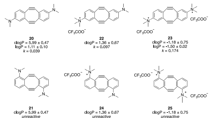
Figure 2. Predicted (clogP) water-solubility values of substituted dialkynes 20-25 . 27 Experimentally determined (logP) values and second-order rate constants ( k , in M -1 s -1 ) indicated below.
