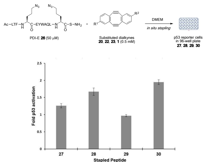
Figure 4. p53 activation in a cellular reporter assay for in situ stapling of peptide 26 (50 \mu M) with substituted dialkynes 20 , 22 , 23 and dialkyne 1 (0.5 mM) in parallel, giving stapled peptides 27 , 28 , 29 , and 30 respectively (performed as technical triplicate). Data reported as fold activation over 1% DMSO. DMEM- Dulbecco's Modified Eagle's Medium.
