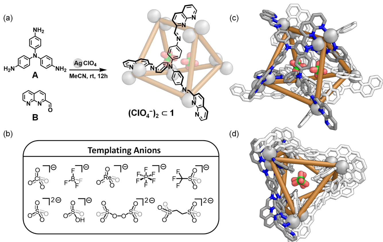
Figure 1. (a) Synthesis of \text{Ag}_{12}\text{L}_6 trigonal prism 1 from tris(4-aminophenyl)amine A , 2-formyl-1,8-naphthyridine B and silver(I) perchlorate. (b) The assembly of 1 requires an appropriate template anion. (c) X-ray crystal structure of (\text{ClO}_4^-)_2 \cdot \mathbf{1} with the two templating anions included. One pair of ligands is shown in gray to highlight the desymmetrization of the ligand arms. (d) Top-down view depicting the central tubular void of (\text{ClO}_4^-)_2 \cdot \mathbf{1} . Disorder, non-included anions and solvent molecules have been omitted for clarity.
