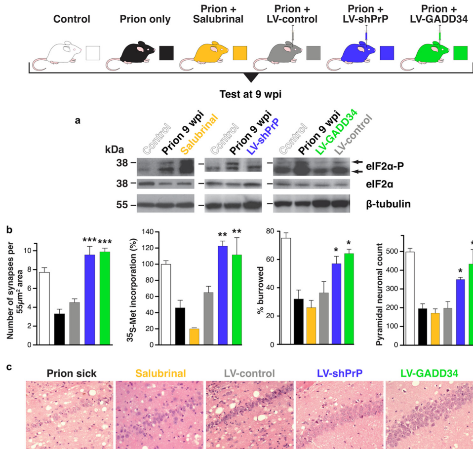
FIGURE 3. Manipulation of the UPR rescues translation and is neuroprotective in prion-diseased mice. a , lentivirally mediated RNAi against PrP (blue bars) or overexpression of GADD34 (green) reduces levels of eIF2 \alpha -P. LV-shPrP, lentivirus mediating RNAi of PrP; LV-GADD34, lentivirus overexpressing the eIF2 \alpha -P phosphatase, GADD34/PP1. b , restoring synapse number, global protein synthesis rates, burrowing behavior, and neuronal cell numbers when compared with untreated prion-diseased mice (black) or empty vector controls (gray). Salubrinal (orange) had a detrimental effect in the same experiments. All data in bar charts show mean \pm S.E. *, p < 0.01 ; **, p < 0.001 ; ***, p < 0.005 . c , neuroprotective effects of RNAi of PrP or GADD34 overexpression in CA1 pyramidal cell ribbon of hippocampus from prion-diseased mice. Adapted from Ref. 33.
