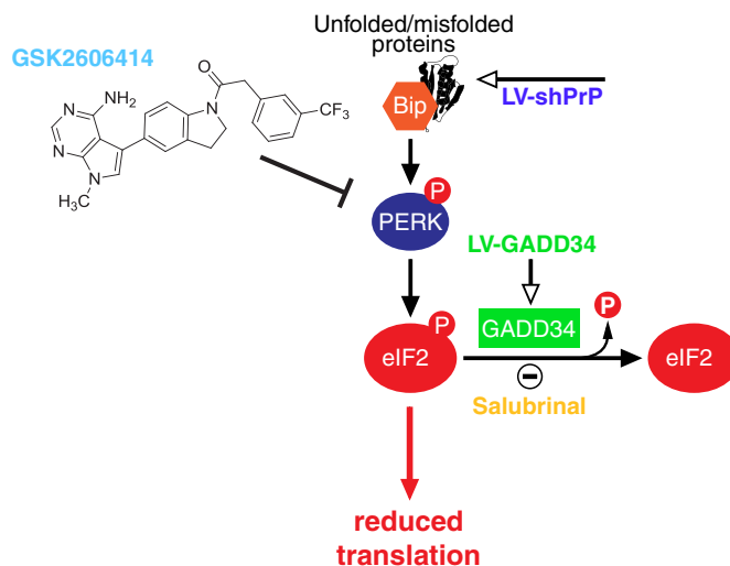
FIGURE 2. Schematic representation of PERK branch of the UPR leading to translational repression and points of intervention. Rising levels of misfolded proteins are detected by binding immunoglobulin protein (BiP) in the ER, activating PERK, which autophosphorylates, and in turn phosphorylates eIF2 \alpha , resulting in reduced translation. The decline in protein synthesis leads to the loss of key proteins, and hence synaptic failure and neurodegeneration. The points of action of GSK2606414, (a specific inhibitor of PERK), of lenticivirus mediating RNAi of PrP (LV-shPrP), and of lenticivirus overexpressing the eIF2 \alpha -P phosphatase, GADD34/PP1 (LV-GADD34) are shown. By inhibiting/preventing PERK phosphorylation (GSK2606414 and LV-shPrP) or dephosphorylating eIF2 \alpha -P (LV-GADD34), protein synthesis is restored. (Salubrinal prevents dephosphorylation of eIF2 \alpha -P, exacerbating the reduction of translation.)
