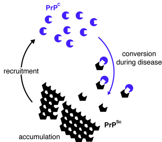
FIGURE 1. Schematic of prion conversion. Native prion protein ( \text{PrP}^{\text{C}} ; blue circular shapes) is converted into \text{PrP}^{\text{Sc}} (black hexagonal shapes) in an autocatalytic process during prion replication. The two proteins have identical primary but different secondary structure. \text{PrP}^{\text{Sc}} is rich in \beta -sheet, is protease-resistant, and accumulates, recruiting more \text{PrP}^{\text{C}} for further cycles of conversion.
