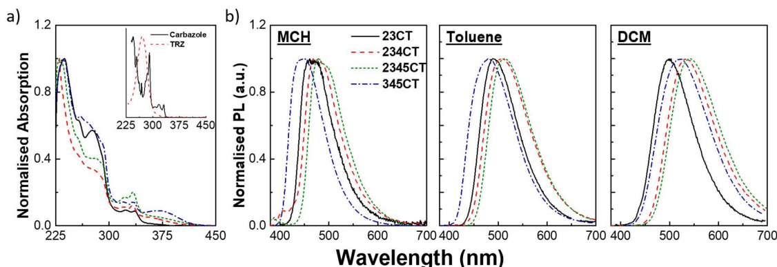
Figure 5.3 – a) Normalised absorption of 23CT, 234CT, 2345CT and 345CT in a dichloromethane (DCM) solution. Inset shows the absorption of the carbazole and TRZ donor and acceptor, respectively. b) Solvatochromic effect on the emission of 23CT, 234CT, 2345CT and 345CT in solvents with increased polarity: MCH, Toluene and DCM. All solutions were excited with 355 nm.
