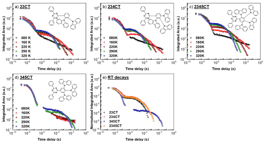
Figure 5.4 – Time-resolved emission decay curves at different temperatures with an excitation of 355 nm and time delays up to 0.03 s of the four emitters in zeonex: a) 23CT, b) 234CT, c) 2345CT, d) 345CT. In e) the normalised decays of each at room temperature are overlaid. The molecular structure of each isomer is shown in the inset of each graph.
