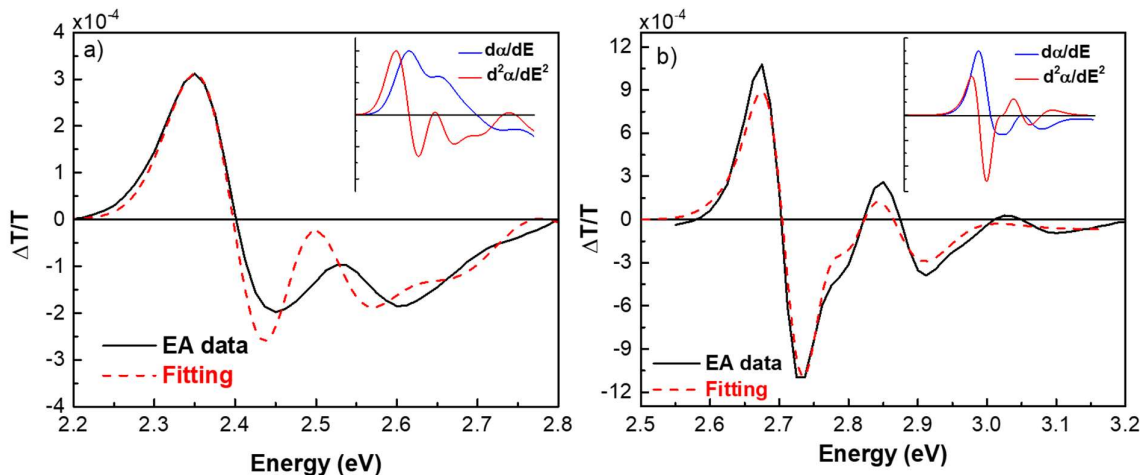
Figure 7.5 – Low energy band Electroabsorption (full black line) spectra of a) POZ-DBPHZ and b) t -BuCz-DBPHZ overlapped with the fitting (dashed red line) using the model described in the Stark Spectra analysis section (Chapter 3). For comparison purposes, the inset of both figures shows the first and second derivatives of the lowest energy absorption bands calculated from the gaussian deconstruction (Figure 7.4).
