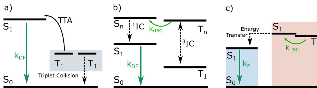
Figure 2.6 – Alternative mechanisms for the generation of DF: a) triplet-triplet annihilation (TTA), b) upper state crossing and c) hyperfluorescence. For simplicity reasons, only the transitions involved in the main mechanisms are shown. In c), two different materials interact with each other, giving rise to energy transfer processes. The blue (left) area refers to a fluorescence-emitting guest and the red (right) to a TADF sensitizer.
