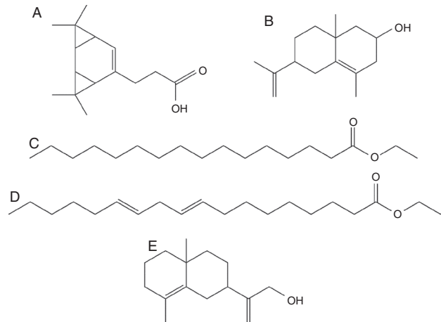
Figure 3: Chemical structures of the major constituents in vetiver root crude extracts and commercial vetiver oil from Vetiveria zizanioides , determined by GC/MS analysis: (A) 3,3,8,8-tetramethyltricyclo[5.1.0.0(2,4)]oct-5-ene-5-propanoic acid; (B) 6-isopropenyl-4,8a-dimethyl-1,2,3,5,6,7,8,8a-octahydronaphthalen-2-ol; (C) ethyl hexadecanoate; (D) ethyl 9,12-octadecadienoate; (E) 2-(4a,8-dimethyl-1,2,3,4,4a,5,6,7-octahydro-naphthalen-2-yl)-prop-2-en-1-ol.
