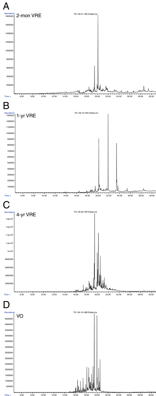
Figure 2: GC-MS spectra of crude Vetiveria zizanioides (vetiver) root ethanol (VRE) extracts and commercial vetiver oil (VO). (A) VRE from greenhouse-grown, 2-mon-old cv. Sierra; (B) VRE from field-grown, 1-yr-old cv. Songkha 3; (C) VRE from greenhouse-grown, 4-yr-old cv. Sierra; (D) commercial VO from Haiti.
