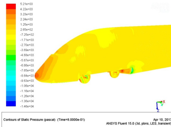
Fig. 8. Static pressure chart of the train head
