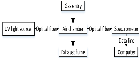
Figure 3. Flow chart of the experimental system.
