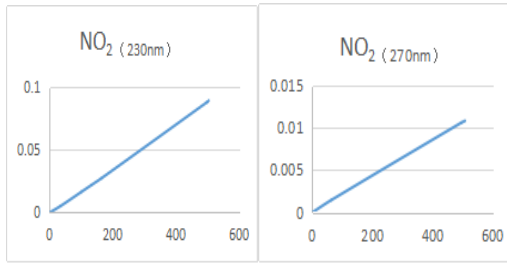
Figure 4. Data relationship between concentration and absorbance of NO 2 .
