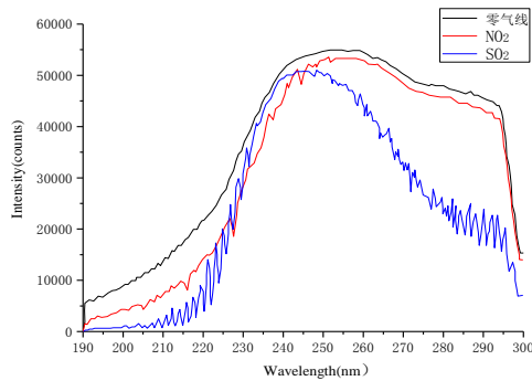
Figure 1. Absorption spectrogram of \text{SO}_2 and \text{NO}_2 .
