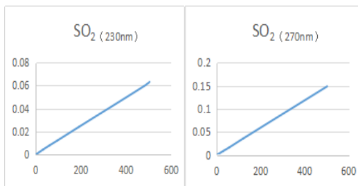
Figure 5. Data relationship between concentration and absorbance of SO 2 .
