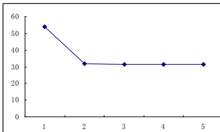
Figure 3. The results of calculation curves of iteration number and SO_2 concentration
