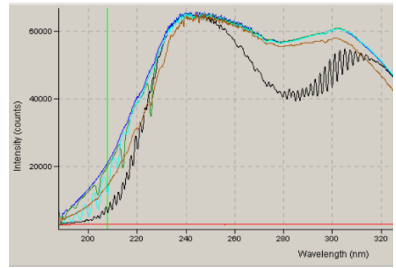
Figure 1. Mixed gas absorption spectrum
