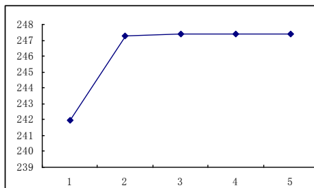
Figure 4. The results of calculation curves of iteration number and NO_2 concentration
