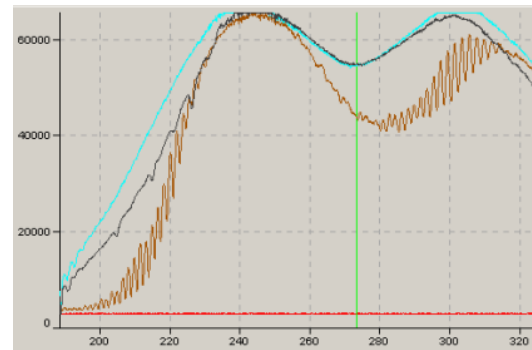
Figure 2. The absorption spectrum of SO_2 and NO_2
