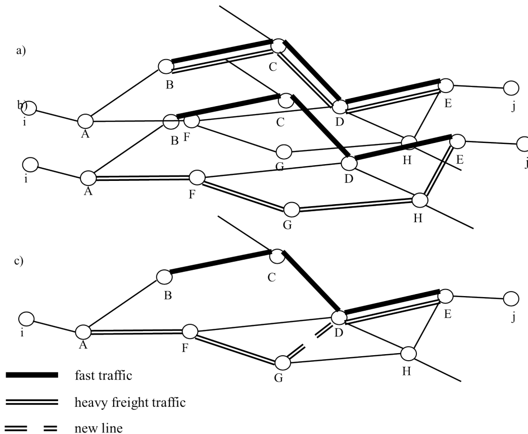
Fig. 2. Principal schemes for the specialization of main railway lines
