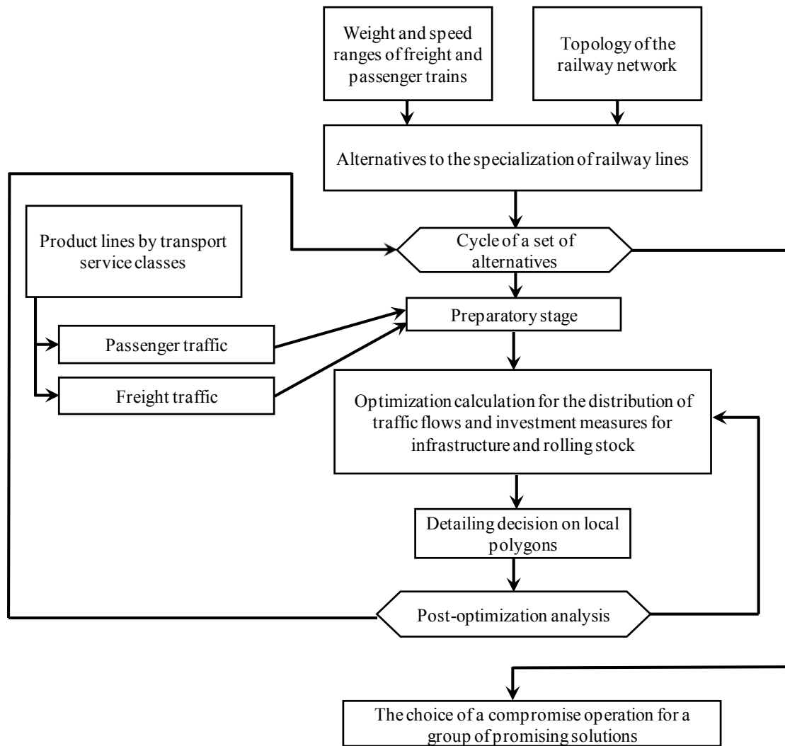
Fig. 3. The general sequence of the search for solving the problem of specialization of railway lines
