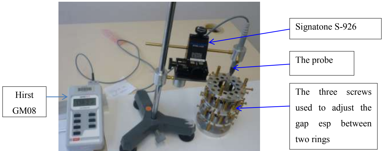
Figure 15: Measurement set-up of the magnetic field in the prototype.
