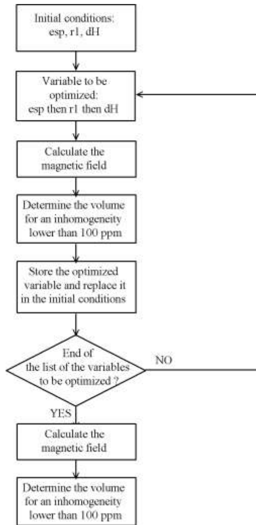
Figure 9: Flow chart of our configuration with 24 main magnets and 8 shim magnets.
