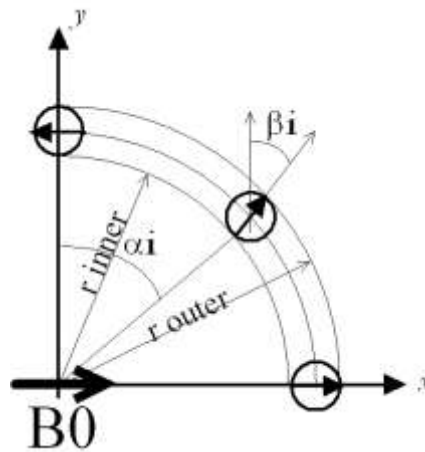
Figure 1: Geometric parameters of Halbach structure.
