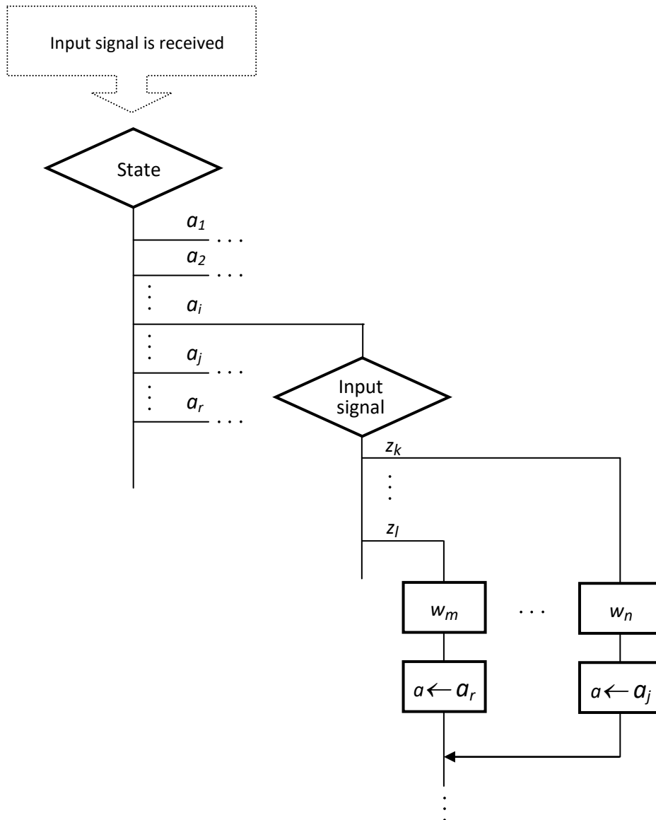
Fig. 4. The fragment of algorithmic diagram of the system response to the receipt of input signal (corresponding to the machine Fig. 3)
