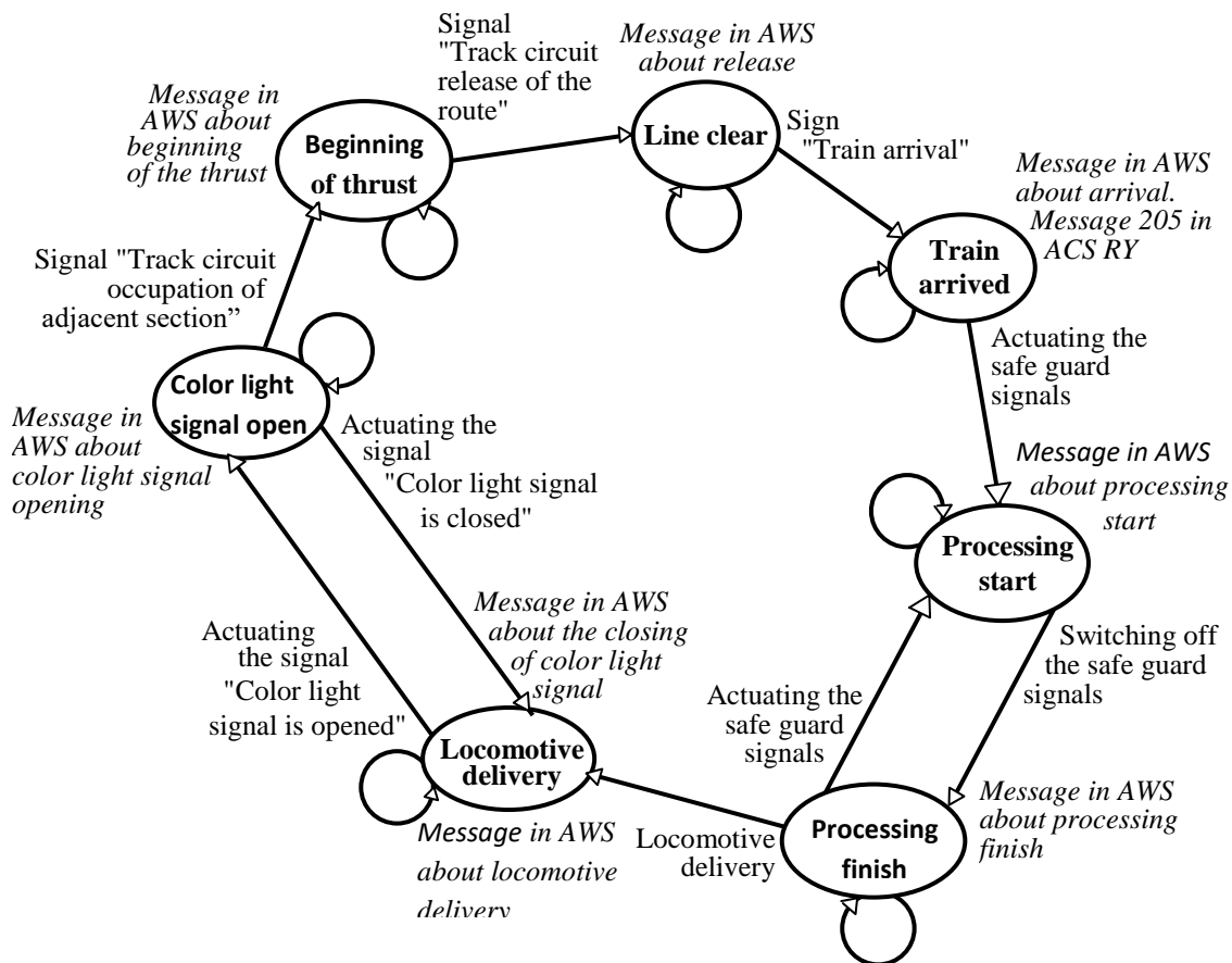
Fig. 2. Part of the automaton representation of information subsystem of the receiving yard
