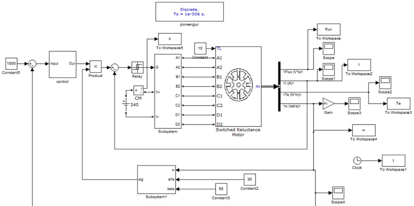
Figure 8. The simulation model of SRM based on fuzzy fractional PID control strategy
