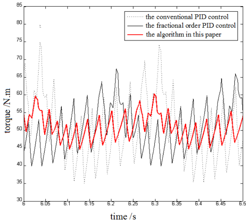
Figure 10. Compared with the output torque of the three algorithms
