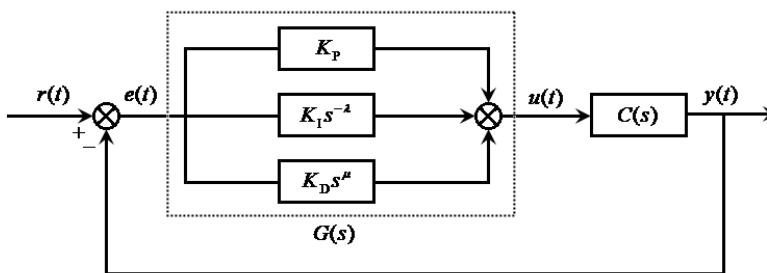
Figure 3. Structure diagram of the fractional order PI^\lambda D^\mu controller
