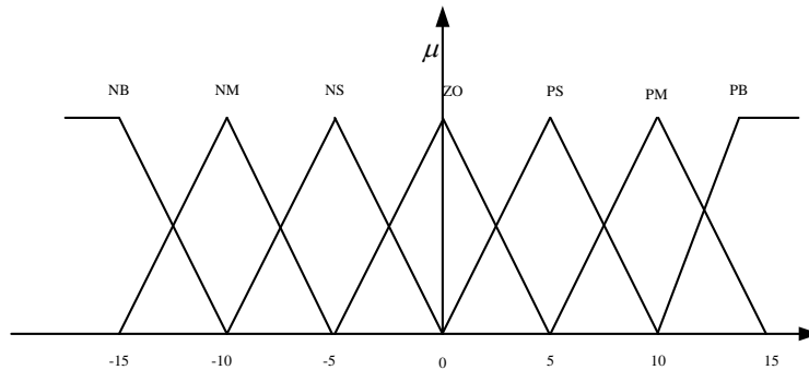
Figure 6. The membership functions of the deviation and the deviation rate \Delta e
