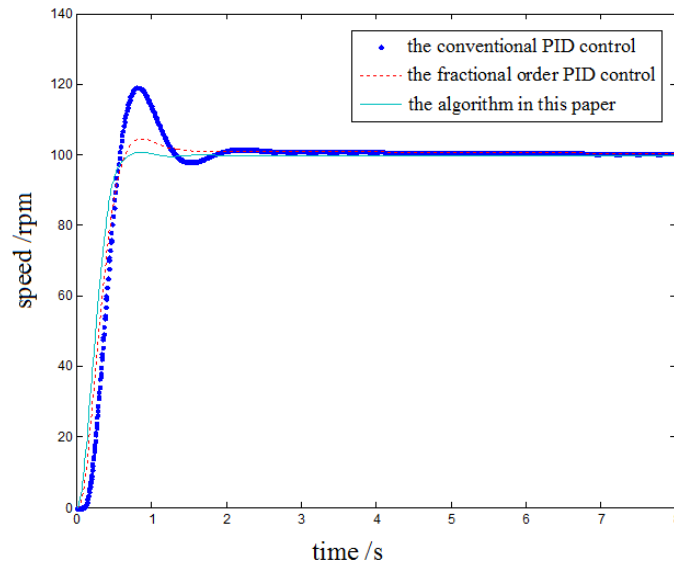
Figure 9. Compared with the step response of the three algorithms
