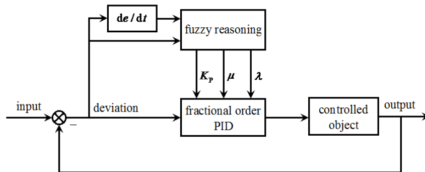
Figure 5. The principle diagram of fuzzy fractional order PID controller
