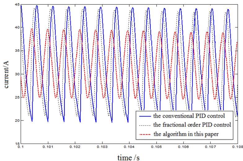
Figure 12. Compared with the current fluctuation of the three algorithms
