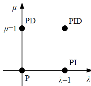
Figure 4(a). Integer order PID controller
