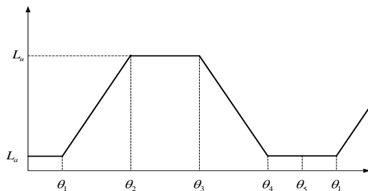
Figure 2. A mathematical model of the equivalent inductance
