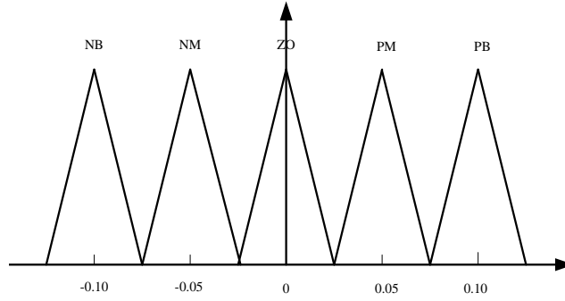
Figure 7. The membership functions of \Delta K_P , \Delta\lambda and \Delta\mu
