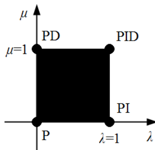
Figure 4(b). Fractional order PID controller
