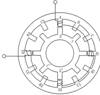
Figure 1. The structure of the SRM
