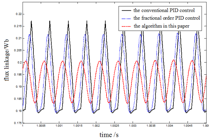
Figure 11. Compared with the flux linkage ripple of the three algorithms
