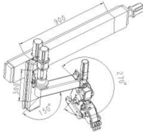
Figure 4. Motion range of robot arm
