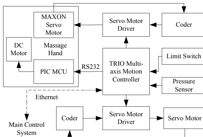
Figure 6. Diagram of motion control system
