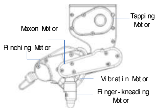
Figure 5. Structure of the massage hand
