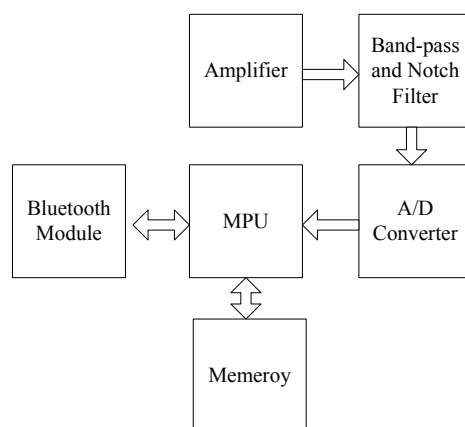
Figure 7. Conceptual architecture of ECG module
