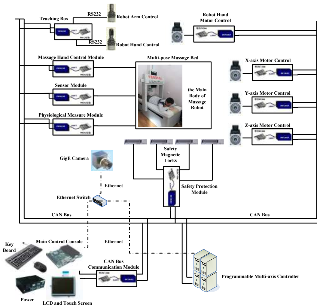
Figure 2. Logic diagram of physiotherapy service robot
