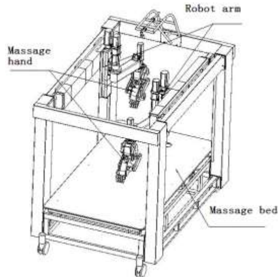
Figure 3. Main body of JZMR-I robot
