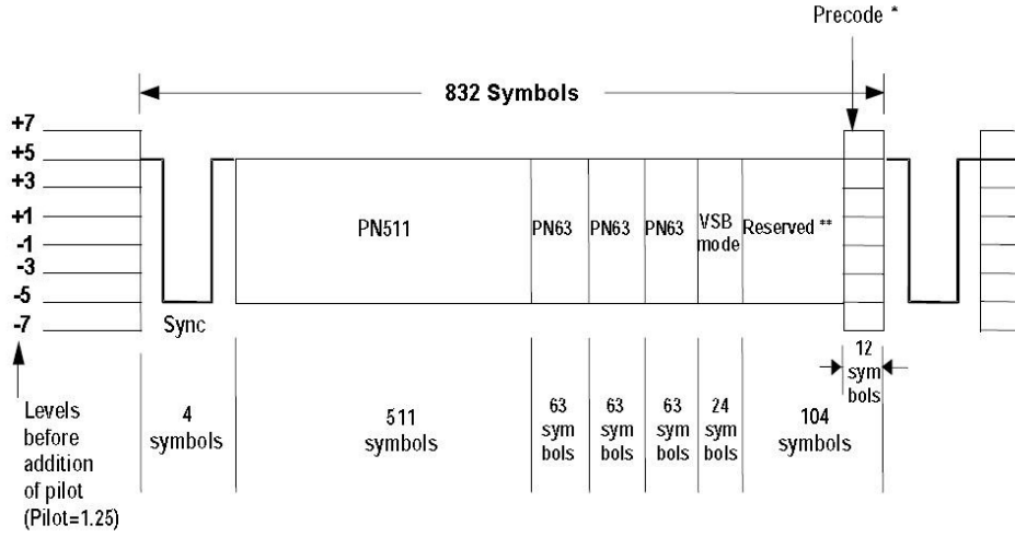
Figure 4. The synchronization of VSB Data Field
