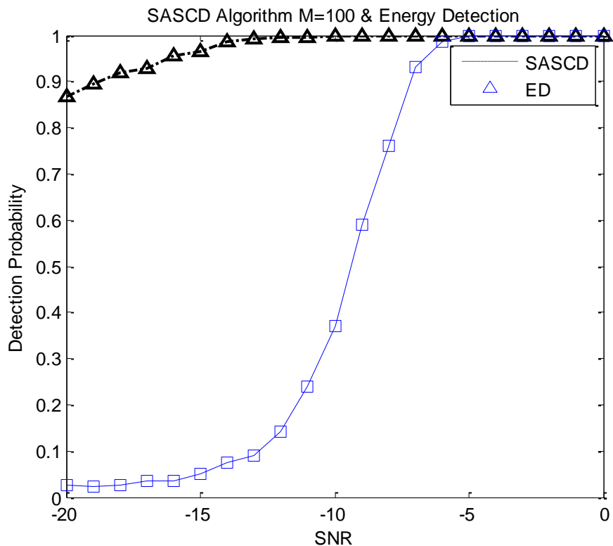
Figure 7. Contrast of SASCD algorithm and energy detection algorithm
