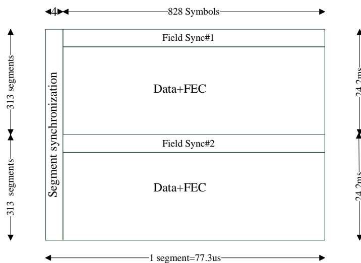
Figure 2. VSB data frame without extra field sync
