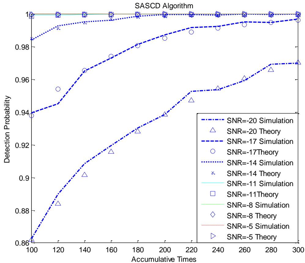
Figure 9. SNR and accumulate more often to the simulation results of the dynamic value
