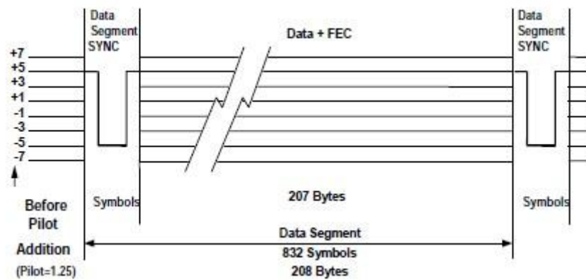
Figure 3. 8-VSB ATSC DTV signal Data Segment
