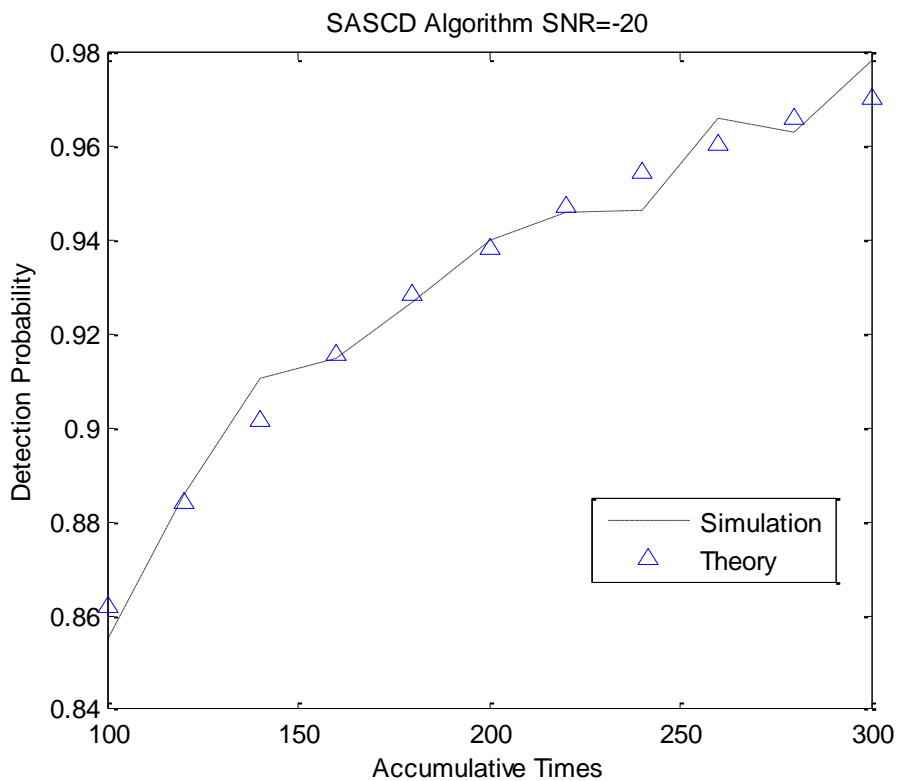
Figure 8. The results of detection propability with fixed SNR
