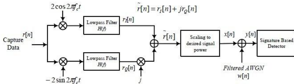
Figure 5. The simulation model of spectrum sensing algorithm based on signal feature
