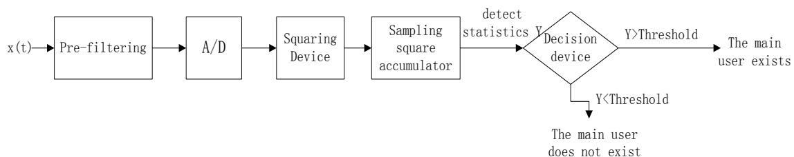
Figure 1. The block diagram of energy detector system
