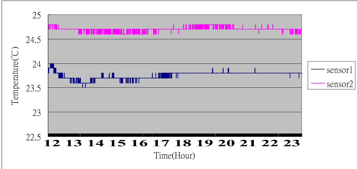
Figure 14. Temperature of FCS (control cycle 10 minutes)
