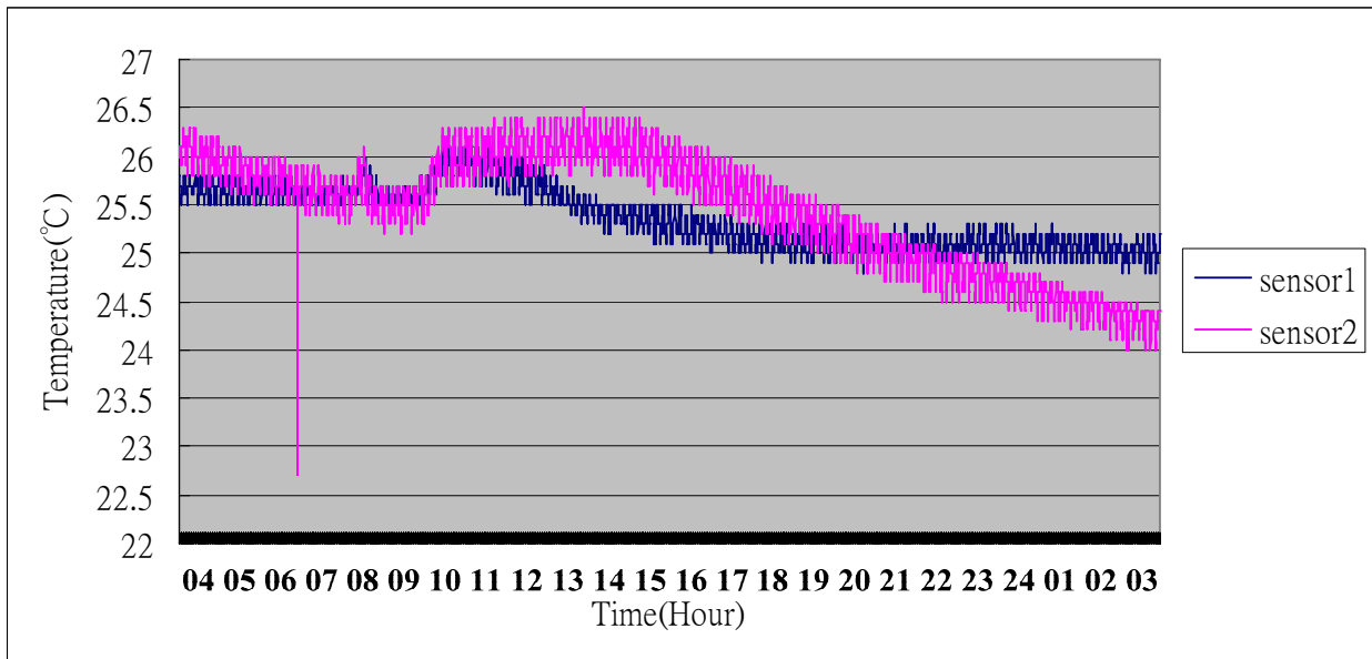
Figure 8. Temperature of FCS
