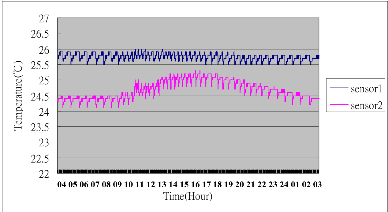
Figure 7. Temperature of TCS
