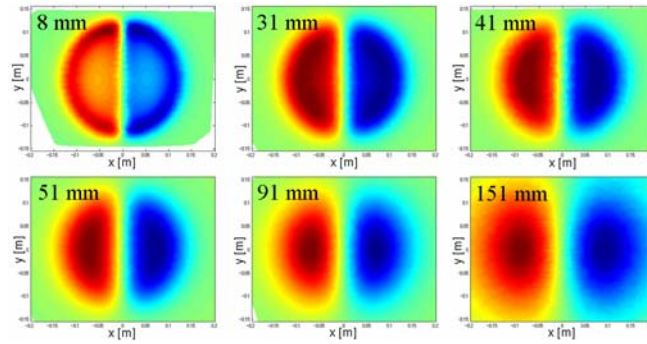
Figure 12. Cut through sensitivity profile of a PMA-2 landmine simulant at various depths. Each image at a given depth has been normalized for better visualization.
