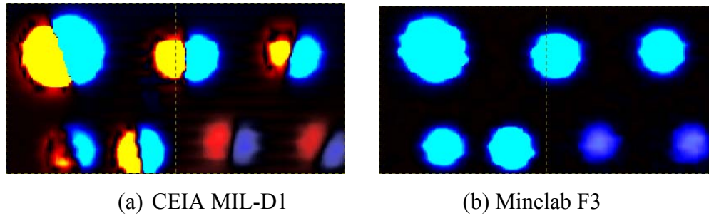
Figure 2: Illustration of imaging of metal detector's sensor data for targets at different depths
