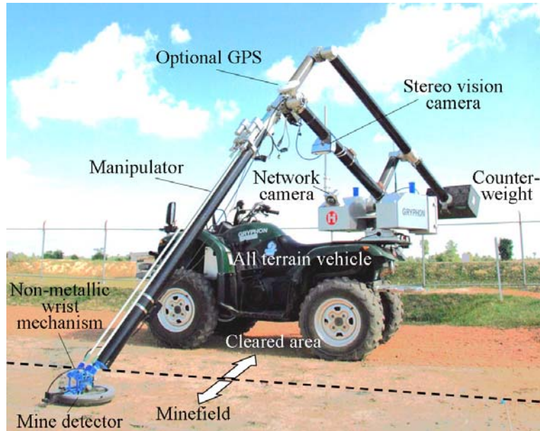
Figure 1: Overview of the Gryphon system.
