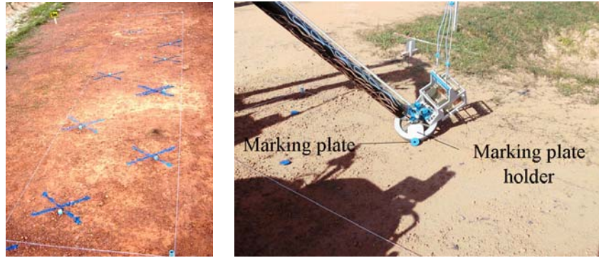
Figure 5. Paint-marked spots and marking plate dropping.
