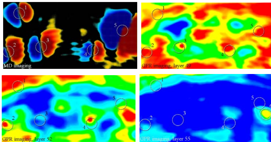
Figure 3: MD and corresponding GPR imaging of a 2 m 2 scan. Buried targets are: 1: PMA-2 at 5 cm depth, 2-4: PMA-1A at 12.5 cm depth, 5: metallic fragment at 5 cm depth and 6: bigger stone at 10 cm depth.
