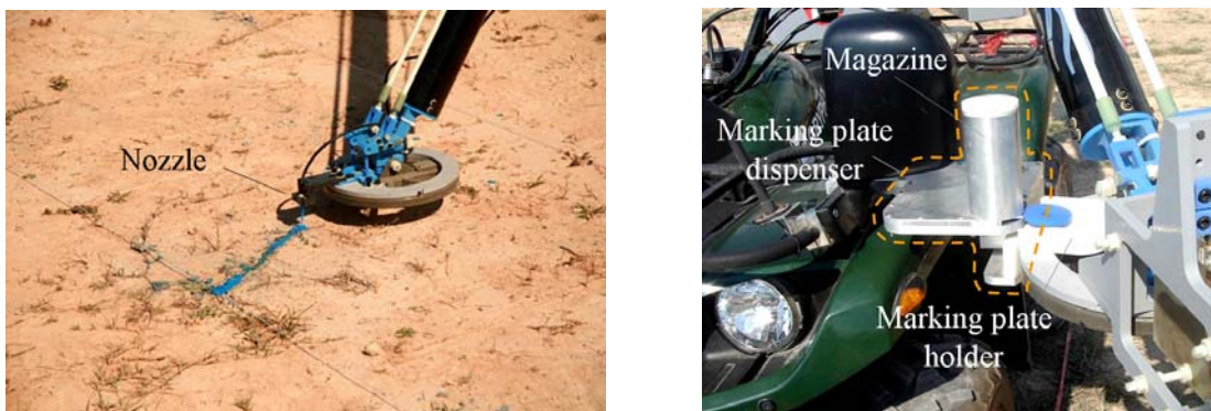
Figure 4: Paint marker and marking plate dispenser.
