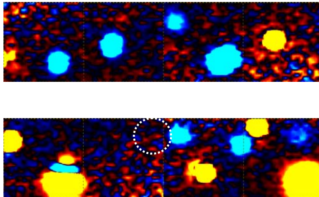
Figure 10. MD images as recorded with the F3-MD-Gryphon. Based on RTK-GPS coordinates, images are automatically appended with the right position/orientation. The adjusted contrast reveals deeply buried objects (indicated with the circle), but at the same time, noise levels also increase.
