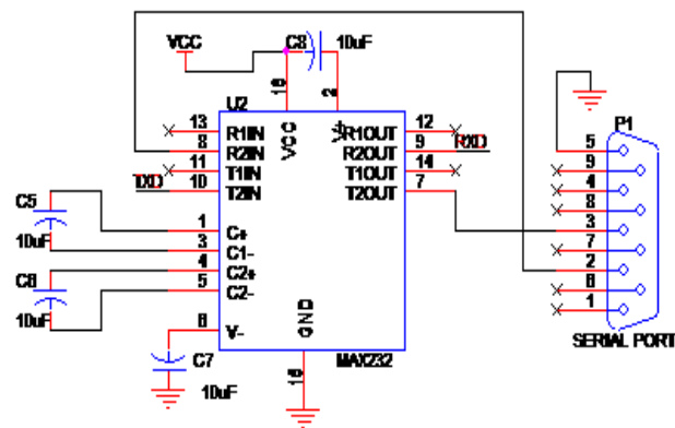
Fig.3 Circuit diagram of RS232 to TTL converter
