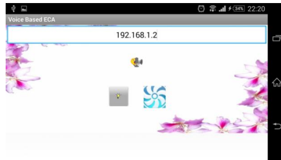
Fig.7 Application output 2
