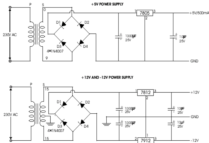
Fig. 2 Circuit Diagram of Power Supply
