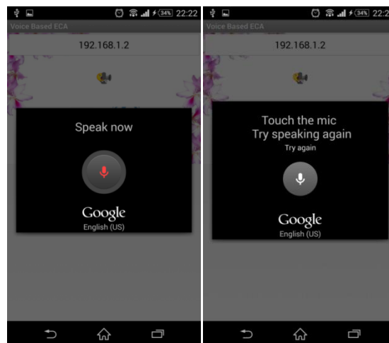
Fig 12 Application output 7
