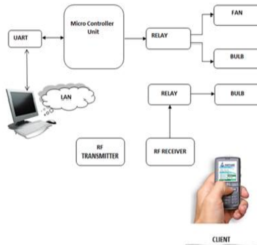
Fig.1 Block diagram of the proposed method
