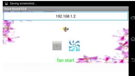
Fig.10 Application output 5
