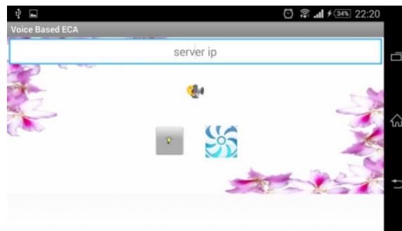
Fig.6 Application Output 1
