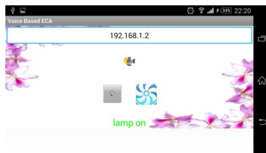
Fig.8. Application output 3
