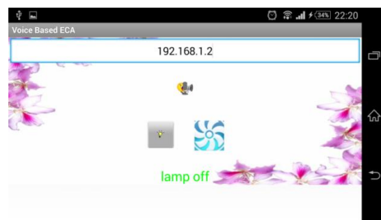
Fig.9 Application output 4
