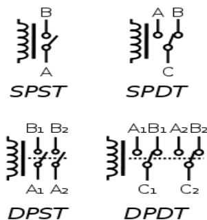
Fig.4 Circuit diagram of relays
