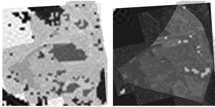
Figure 2. Composite pictures with the given limit temperature 33°C and 41°C by earlier spring case
