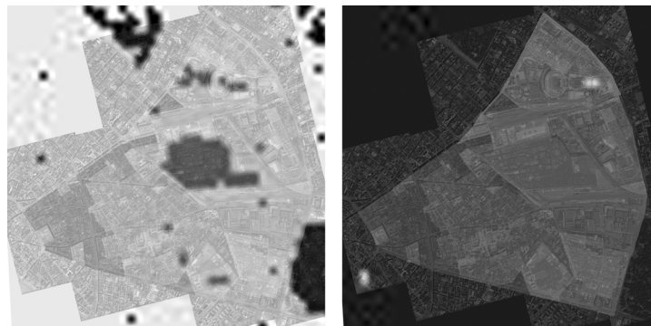
Figure 3. Composite pictures with the given limit temperature -3°C and 2°C by the winter case
