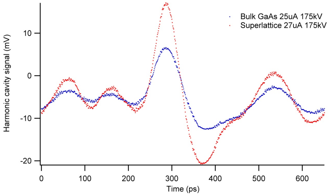
Figure 2.6.7: Harmonic cavity signals for a 25 uA, 175 kV beam.
