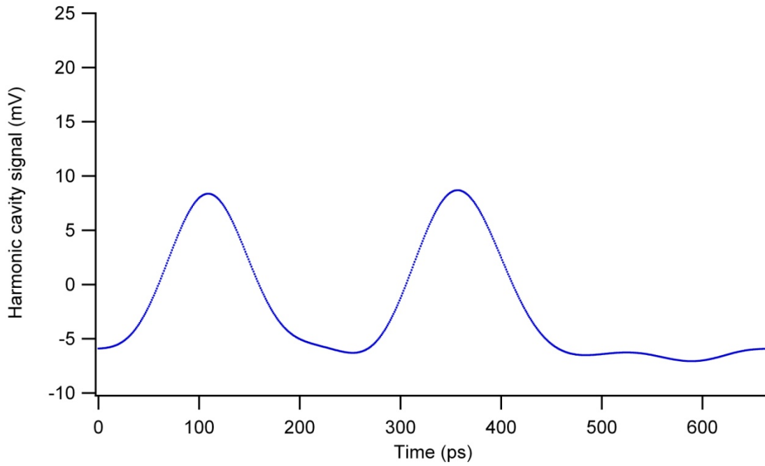
Figure 3.9.4: Processed waveform is near 90° from bunch coincidence.
