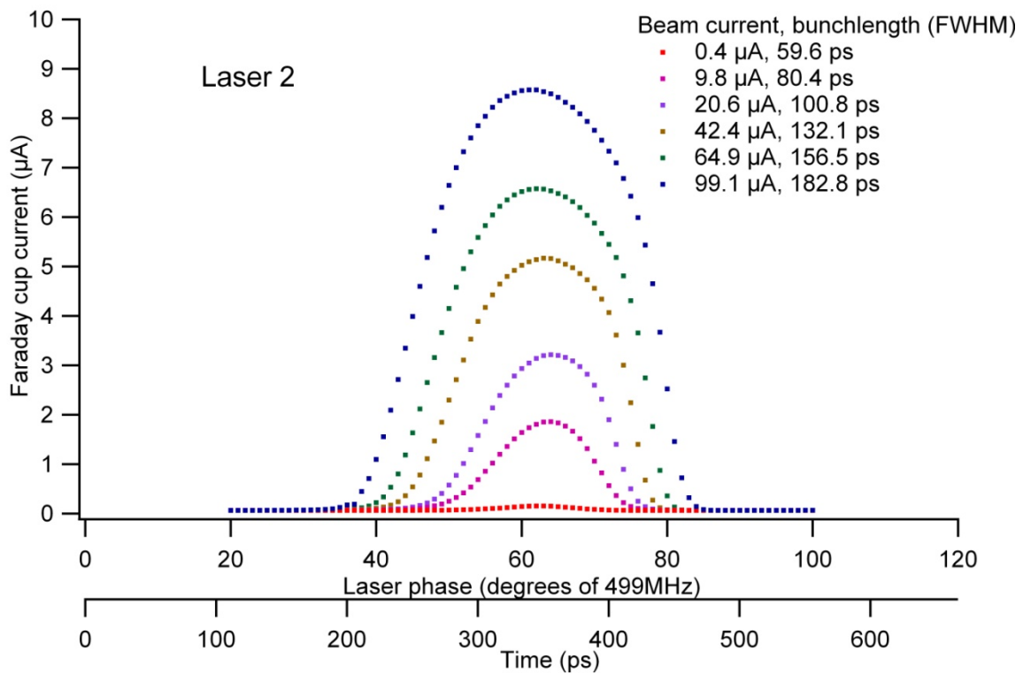
Figure 3.7.1: Deflection measurements of the 249.5 MHz beam.
