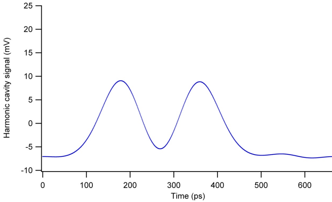
Figure 3.9.6: Processed waveform is near 60^\circ from bunch coincidence.
