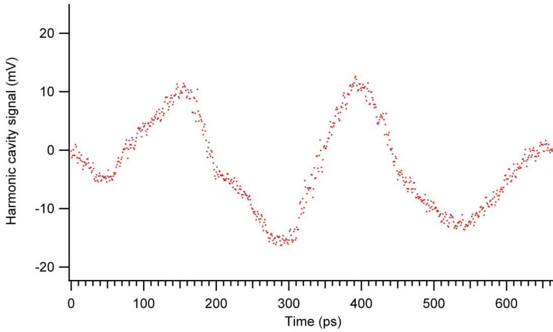
Figure 3.9.3: Two interleaved 499 MHz beams about 30° out of phase.
