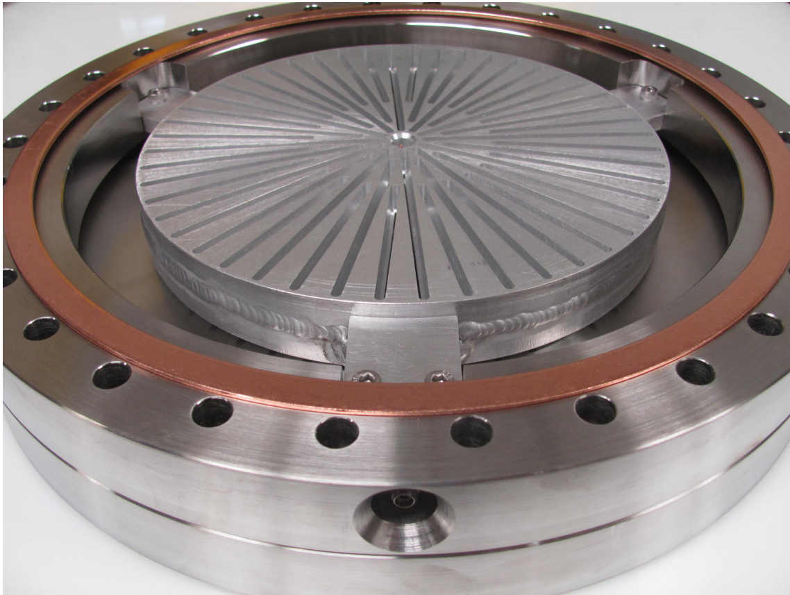
Figure 1.1.5: A beamline compatible harmonic cavity constructed for testing on the Jlab Injector Test Facility.
