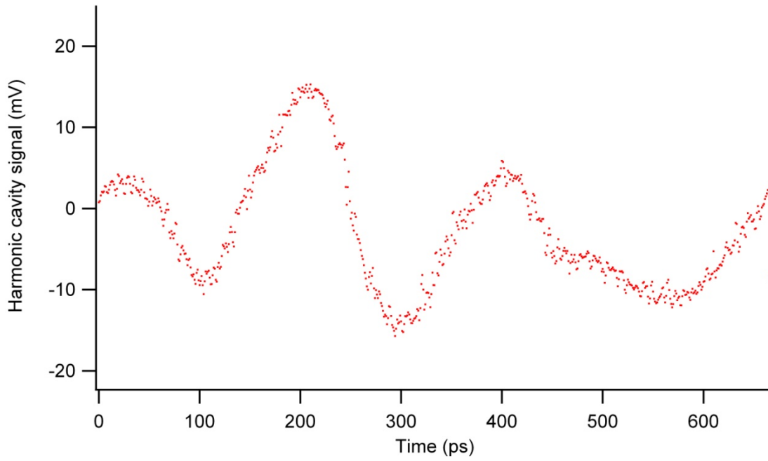
Figure 3.9.5: Two interleaved 499 MHz beams about 20^\circ out of phase.
