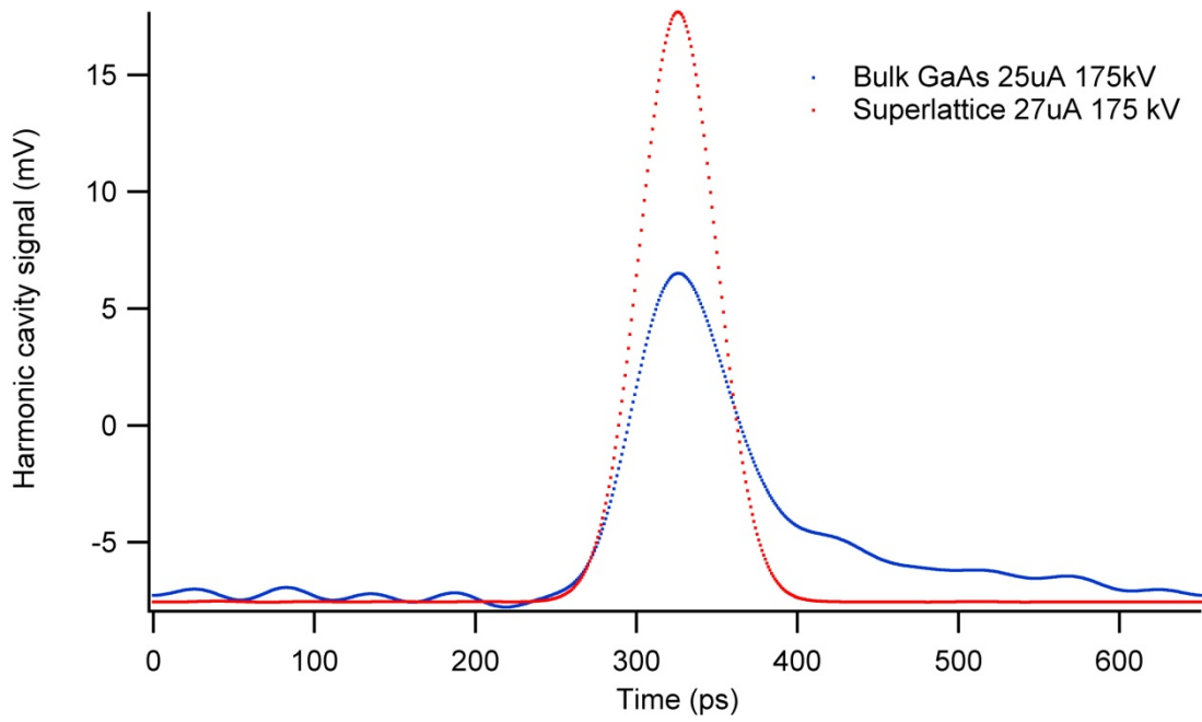
Figure 2.6.8: Processed signals for a 25 uA, 175 kV beam.
