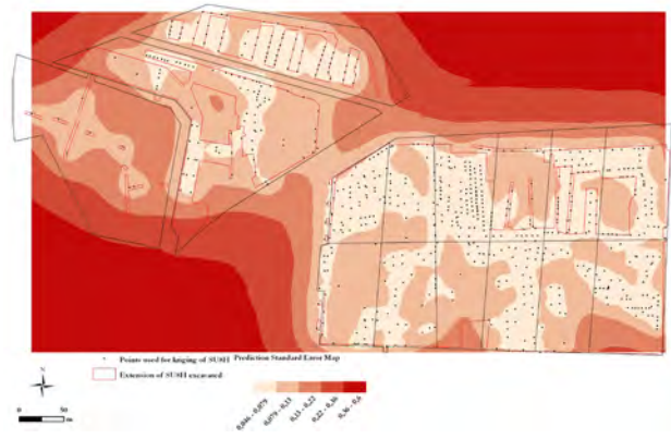
FIGURE 6: STANDARD PREDICTION ERROR MAP OF THE DEM (FIGURE 5)
