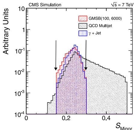
Fig. 4. Normalized distribution of S_{\text{Minor}} for simulated signal, \gamma + jets, and QCD multijet events. The arrows indicate the S_{\text{Minor}} selection interval. (For interpretation of the references to color in this figure legend, the reader is referred to the web version of this Letter.)
