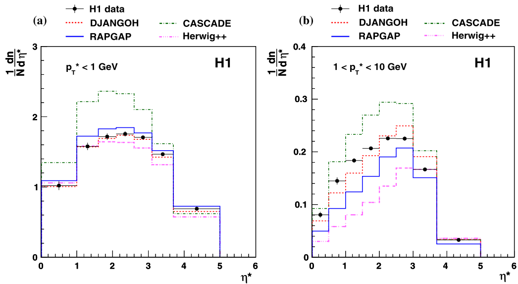
Fig. 5 Charged particle density as a function of \eta^* for (a) p_T^* < 1 \text{ GeV} for (b) 1 < p_T^* < 10 \text{ GeV} compared to DJANGO, RAPGAP, Herwig++ and CASCADE Monte Carlo predictions
