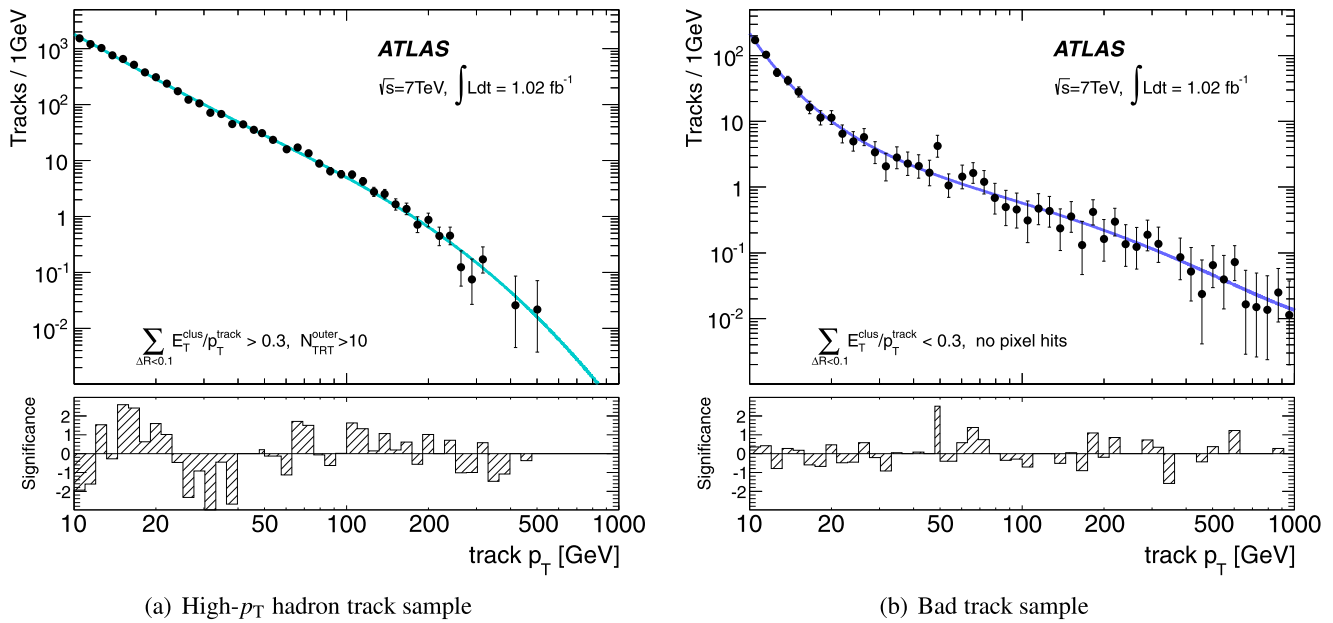
Fig. 3 The p_T distributions of high- p_T hadron track (a) and bad track (b) background control samples. The data and the fitted model are shown by the solid circles and the line , respectively. The significance
