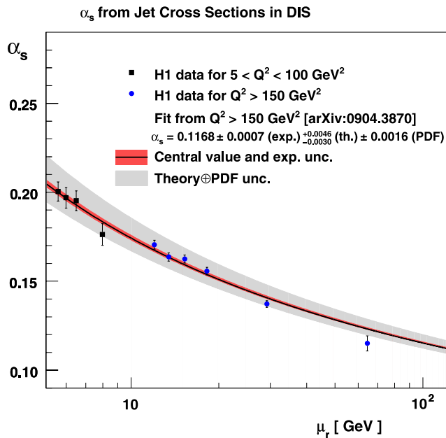
Fig. 12 Values of \alpha_s(\mu_r = \sqrt{(Q^2 + P_{T,\text{obs}}^2)/2}) obtained by a simultaneous fit of all jet cross sections in each Q^2 bin of this analysis ( squares ) together with the fit in different bins at high Q^2 ( circles ) [4]. The solid line shows the two loop solution of the renormalisation group equation obtained by evolving the \alpha_s(M_Z) extracted from jets at high Q^2 . Other details are given in the caption to Fig. 9
