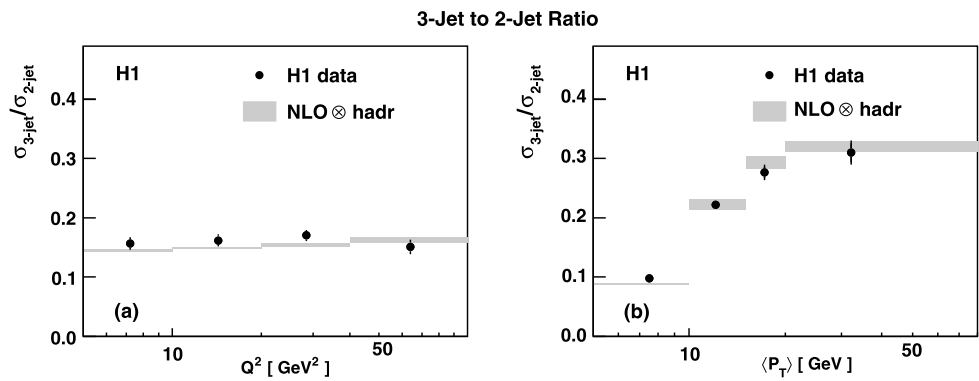
Fig. 7 Ratios of 3-jet to 2-jet cross sections as a function of Q^2 (a) and \langle P_T \rangle integrated over the full Q^2 range (b) compared with NLO QCD predictions corrected for hadronisation. Other details are given in the caption to Fig. 2
