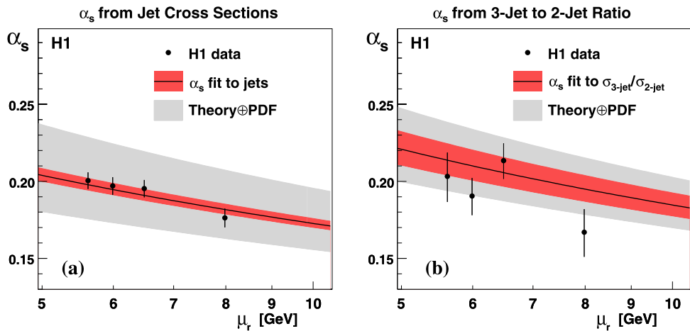
Fig. 11 Values of \alpha_s(\mu_r = \sqrt{(Q^2 + P_{T,\text{obs}}^2)/2}) obtained by a simultaneous fit of all jet cross sections in each Q^2 bin (a) and of the ratio of 3-jet cross section to 2-jet cross section (b). The solid lines show the two loop solution of the renormalisation group equation obtained by evolving the \alpha_s obtained from these measurements. For (a) the value of \alpha_s is extracted from a simultaneous fit of 62 measurements of inclusive jet, 2-jet and 3-jet double differential cross sections in bins
