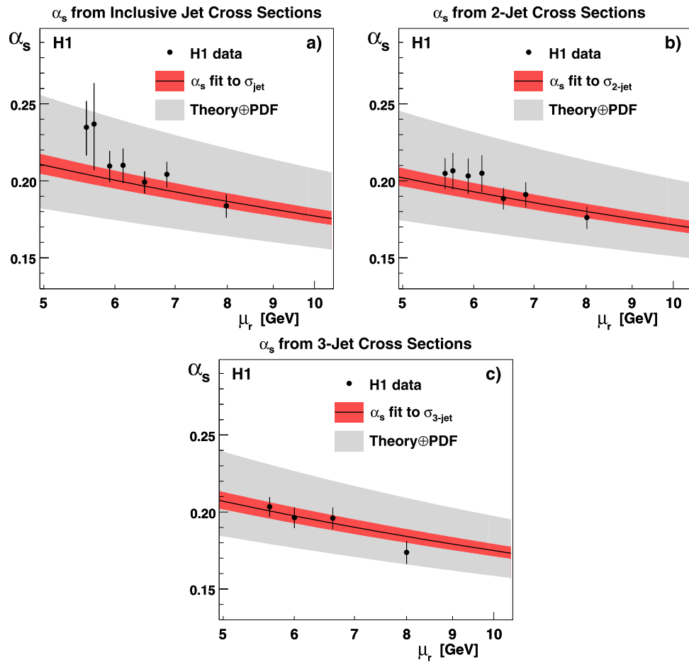
Fig. 10 Values of \alpha_s(\mu_r = \sqrt{(Q^2 + P_{T,\text{obs}}^2)/2}) extracted from inclusive jet cross section (a), 2-jet cross section (b), and 3-jet cross section (c). In each case, the solid lines show the two loop solution of the
