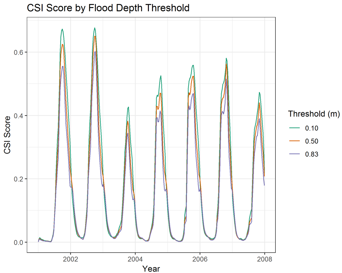
Figure 3-14 Critical Success Index (CSI) score by flood depth thresholds of 0.1 m, 0.5 m and 0.83 m for the All Bathymetry + Width model. CSI scores calculated over a 7-year period (2001-2007) at the time of the MODIS observations (approximately every 8 days; Total 322 images). A CSI score of 1 indicates a perfect match between simulated and observed flood extent, whilst a CSI score of 0 indicates no match between simulated and observed flood extent.
