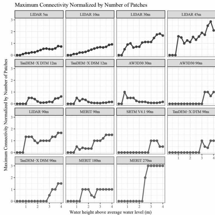
Figure 5-14 Maximum Connectivity (number of connections) normalized by number of patches for all DEMs for D4 and D8 connectivity. Maximum MERIT connectivity refers to the maximum DTM number of times a floodplain cell is connected to breached bank pixels. See Figure 5-11 for a schematic of Maximum connectivity.
