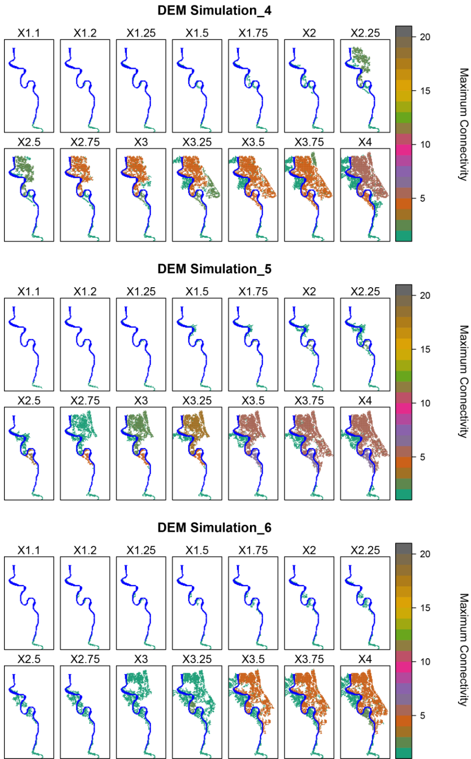
Figure 5-31 Maximum Connectivity (Number of river-floodplain connections per patch) for D8 connectivity for 3 Simulated MERIT DEMs (Sample 1)
