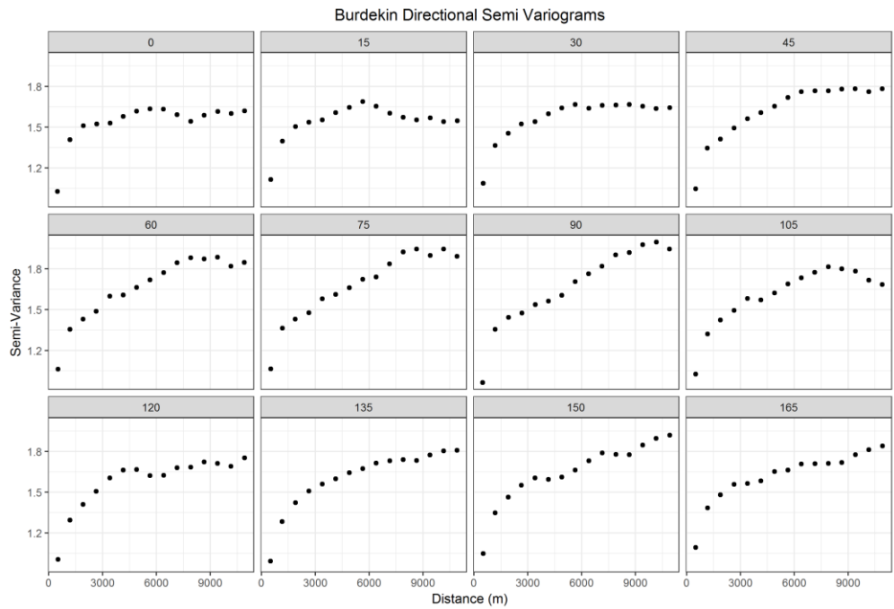
Figure 4-10 Directional semi-variograms for Burdekin. The number in each panel refers to the degrees from north, when north=0 and east=90. There is better long-range spatial continuity (smaller semi-variance values) in the North (0) and North-East directions
