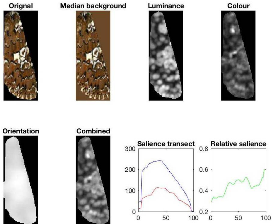
Figure 2.5 An example of the output from the wing saliency computer program for the right wing of the white spot ( Hadena albimacula ), this program being an adaptation of Rosenholtz et al. 's (2005, 2007) code for measuring visual clutter. From left to right: the original image file, the file with background set to the median colour of the wing, a saliency map based on luminance contrast, a saliency map based on colour contrast, a saliency map based on orientation contrast, a combined saliency map, a transect along the combined saliency map, showing the sum of saliency values (red line) and available wing area (blue line) in each vertical column when moving from left to right along the wing, a transect of the saliency score relative to the available wing area when moving from left to right along the wing.
