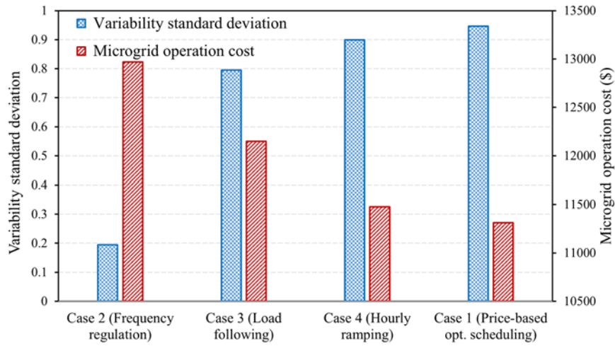
Fig. 3.9. Standard deviation of distribution feeder net load variabilities versus microgrid operation cost for studied cases.
