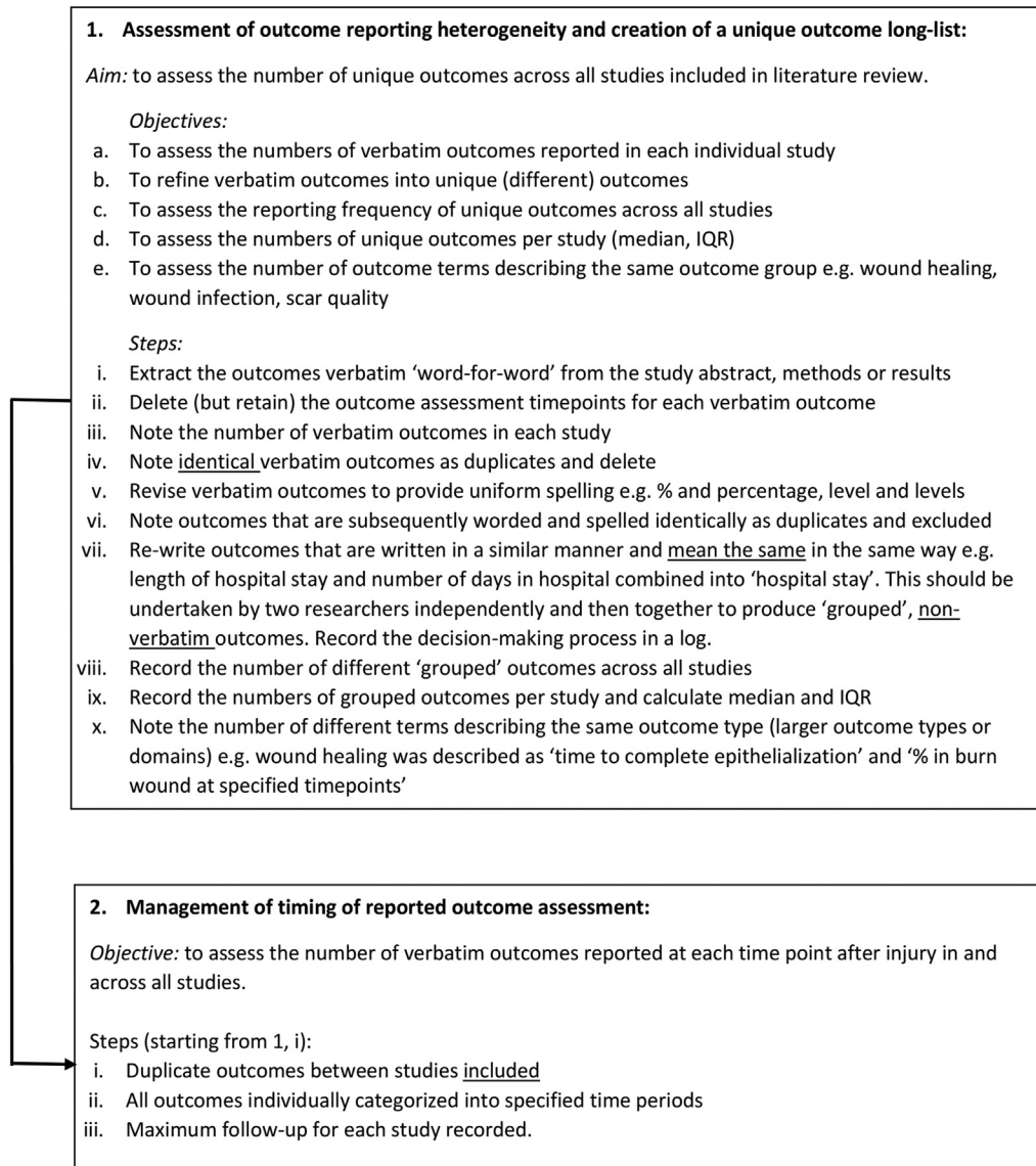
Fig. 3. Unique outcome methodology proposal.
