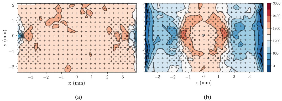
Fig. 5. 2D elastic strain ( \epsilon_{yy} ) fields acquired using XRD at an applied load of 4 kN for (a) a/W = 0.1 ; (b) a/W = 0.5 .
